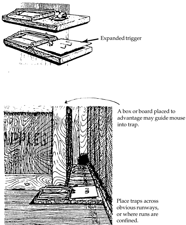
Fig. 15. Expanded-trigger traps, when properly placed, can be very effective.
