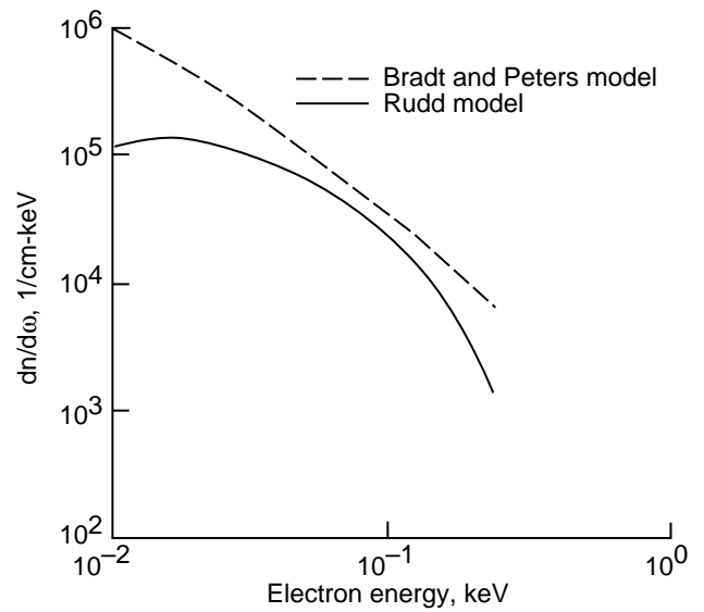
(b) Spectrum with 0.1 MeV proton in water.
