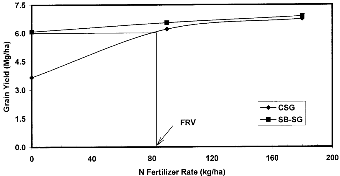
Fig. 2. Average sorghum grain yield response to N fertilizer applications in continuous sorghum (CSG) and soybean-sorghum (SB-SG) rainfed cropping systems at Mead, NE (1983–2002). FRV, fertilizer replacement value.
