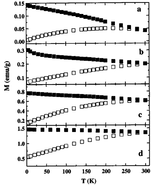
FIG. 10. Field-cooled (solid squares) and zero-field-cooled (open squares) magnetization at 100 Oe for (a) \text{Ni}_3\text{C} after 90 h of mechanical alloying and the same sample annealed at (b) 200 °C for 1 h, (c) 350 °C for 1 h, and (d) 350 °C for 5 h.
