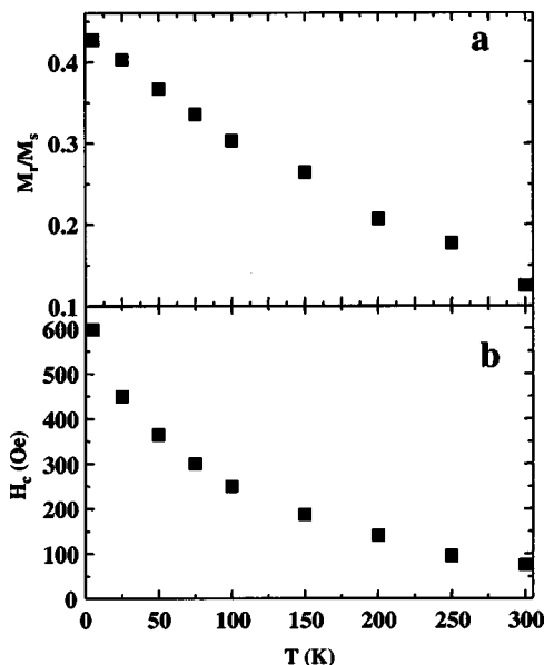
FIG. 9. (a) Remanence ratio and (b) coercivity as functions of temperature for \text{Ni}_3\text{C} after 90 h of mechanical alloying.
