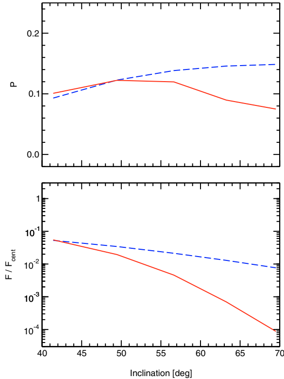
Fig. 8. Differences between large and small tori with an elliptical cross-section in the V-band (see Sect. 4.2). Top : polarization, P , and bottom , the fraction, F/F_{\text{cent}} , of the central flux, F_* , as a function of viewing inclinations, i . The dashed lines denote the thin elliptical torus (case 2), the solid line the extended torus (case 3)
