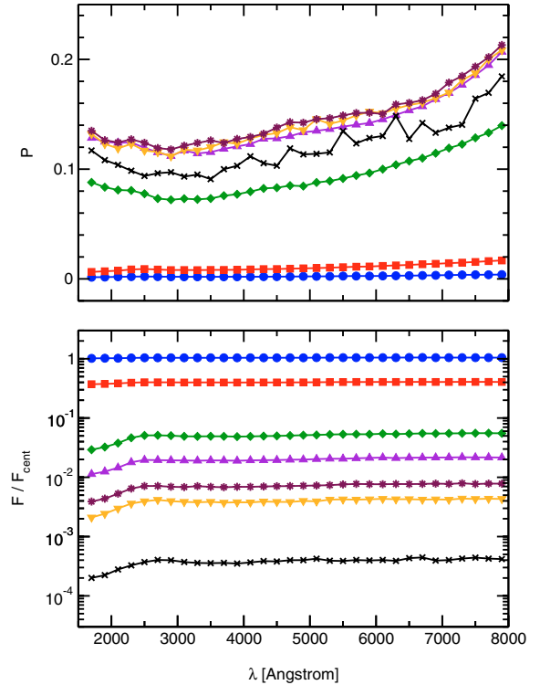
Fig. 5. Modeling a cylindrical torus with an elliptical cross-section and \theta_0 = 30^\circ (see Sect. 4.1). Top : polarization, P . Bottom : the fraction, F/F_{\text{cent}} , of the central flux, F_* , seen at different viewing inclinations, i . Legend: i = 87^\circ (edge-on) (black crosses), i = 76^\circ (orange triangles with points down), i = 70^\circ (intermediate) (maroon stars), i = 57^\circ (purple triangles with points up), i = 41^\circ (green diamonds), i = 32^\circ (red squares), and i = 18^\circ (face-on) (blue circles).
