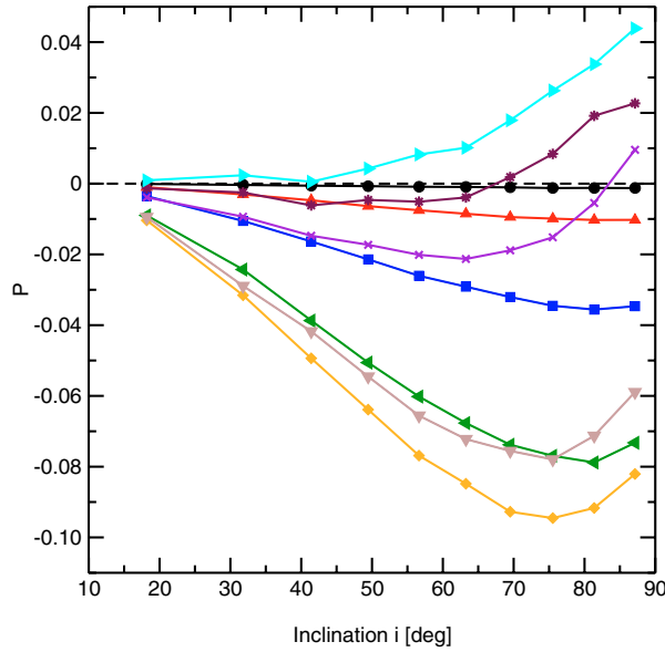
Fig. 16. Same parameters as in Fig. 15, but for a thin disk with \frac{h}{a} = 0.01 . Legend: \tau_{\text{ES}} = 0.001 (black circles), \tau_{\text{ES}} = 0.01 (red triangles with points up), \tau_{\text{ES}} = 0.05 (blue squares), \tau_{\text{ES}} = 0.2 (green triangles with points left), \tau_{\text{ES}} = 0.5 (orange diamonds), \tau_{\text{ES}} = 1 (brown triangles with points down), \tau_{\text{ES}} = 3 (purple crosses), \tau_{\text{ES}} = 5 (maroon stars), and \tau_{\text{ES}} = 10 (cyan triangles with points right).
