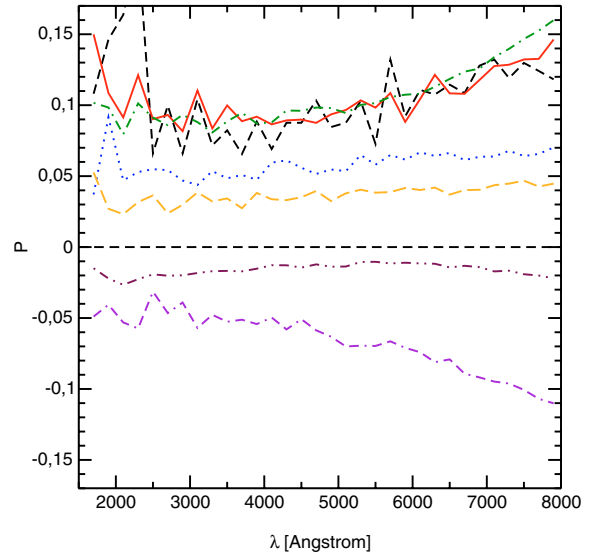
Fig. 9. Polarization averaged over type-2 viewing angles (see Sect. 4.3). A positive value of polarization denotes an E -vector oriented perpendicular to the torus symmetry axis; for negative values the E -vector is aligned with the projected axis. Legend: \theta_0 = 10^\circ (black dashed line), \theta_0 = 20^\circ (solid red line), \theta_0 = 30^\circ (green dot-dashed line), \theta_0 = 45^\circ (blue dots), \theta_0 = 50^\circ (long yellow dashes), \theta_0 = 60^\circ (brown double dots and dashes), and \theta_0 = 75^\circ (pink double-dashes and dots).
