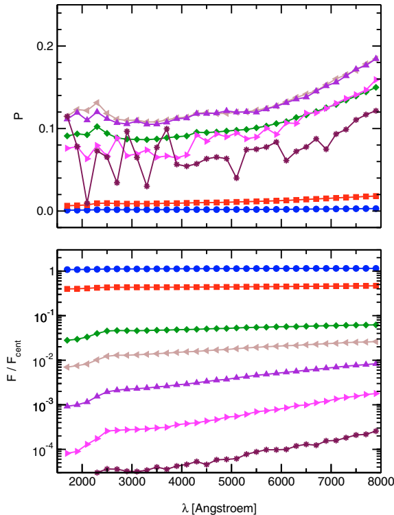
Fig. 6. Modeling a large torus with an elliptical cross-section and \theta_0 = 30^\circ (see Sect. 4.2). Top : polarization, P . Bottom : the fraction, F/F_{\text{cent}} , of the central flux, F_* , seen at different viewing inclinations, i . Legend: i = 70^\circ (intermediate) (maroon stars), i = 63^\circ (pink triangles with points to the right), i = 57^\circ (purple triangles with points up), i = 49^\circ (brown triangles with points to the left), i = 41^\circ (green diamonds), i = 32^\circ (red squares), and i = 18^\circ (face-on) (blue circles)
