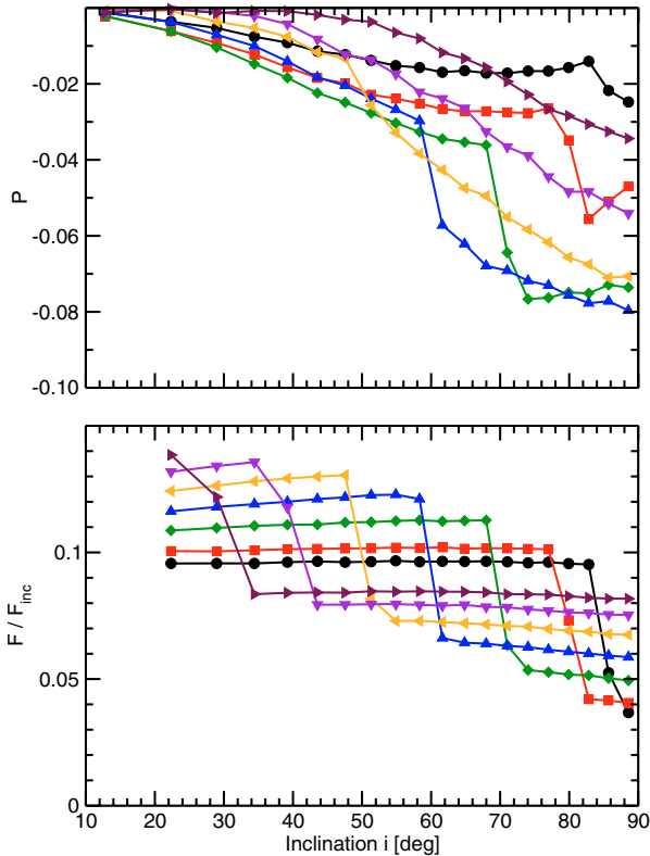
Fig. 18. Modeling equatorial flared scattering disks of various half-opening angles \theta_D (see Sect. 6.2.1). Top : polarization, P , with negative values denoting type-1 polarization (parallel to the symmetry axis). Bottom : the fraction, F/F_{\text{inc}} , of the central flux, F_* , plotted versus inclination, i , with respect to the observer. The different symbols denote different half-opening angles of the flared disk. Legend: \theta_D = 5^\circ (black circles), \theta_D = 10^\circ (red squares), \theta_D = 20^\circ (green diamonds), \theta_D = 30^\circ (blue triangles with points up), \theta_D = 40^\circ (orange triangles with points to the left), \theta_D = 50^\circ (purple triangles with points down), and \theta_D = 60^\circ (brown triangles with points to the right).
