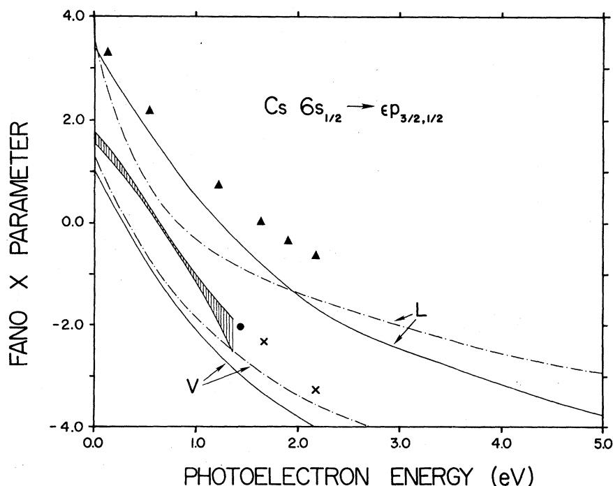
FIG. 6. Fano parameter X(E) vs photoelectron energy (eV); —, present relaxed-core results in dipole-length ( L ) and dipole-velocity ( V ) approximation; - · -, present frozen-core results in dipole-length ( L ) and dipole-velocity ( V ) approximation; shaded band, experimental results of Baum et al. (Ref. 9); ●, semiempirical calculation of Norcross (Ref. 16); ×, semiempirical calculation of Weisheit (Ref. 15); ▲, Dirac-Fock calculation of Chang and Kelly (Ref. 18).
