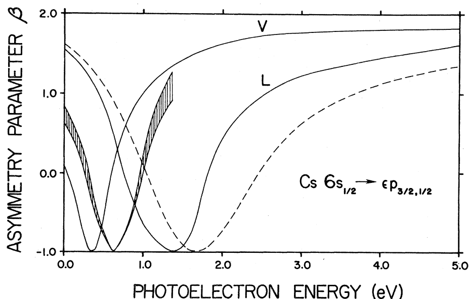
FIG. 3. Angular distribution asymmetry parameter \beta(E) vs photoelectron energy (eV): —, present relaxed-core results in dipole-length (L) and dipole-velocity (V) approximation; shaded band, inferred experimental results obtained from data of Baum et al. (Ref. 9) for X(E) ; ---, Dirac-Fock calculation of Ong and Manson (Ref. 20).
