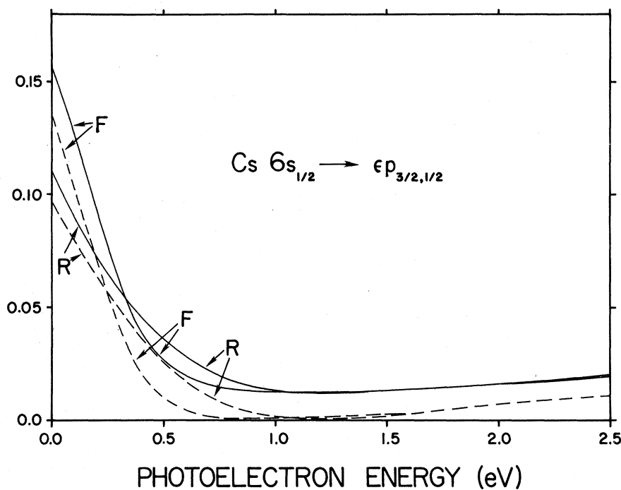
FIG. 1. Cross section for photoionization of the 6s electron in cesium vs photoelectron energy (eV): ---, HF results; —, results including effect of spin-orbit interactions. Results are presented in both the frozen-core approximation (F) and the relaxed-core approximation (R). For clarity, only dipole-length results are shown.
