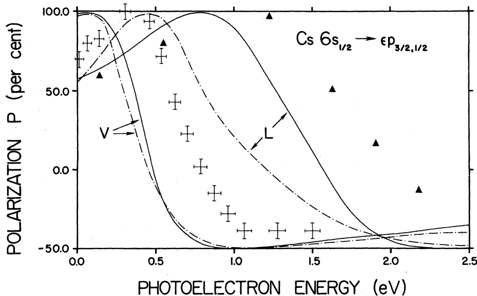
FIG. 5. Photoelectron spin polarization parameter P(E) vs photoelectron energy (eV): —, present relaxed-core results in dipole-length ( L ) and dipole-velocity ( V ) approximation; -·-, present frozen-core results in dipole-length ( L ) and dipole-velocity ( V ) approximation; crosses, experimental results of Heinzmann et al. (Ref. 8); \blacktriangle Dirac-Fock calculation of Chang and Kelly (Ref. 18).
