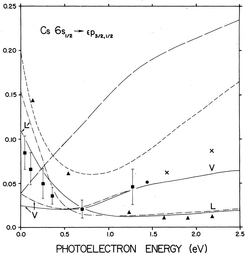
FIG. 2. Cross section for photoionization of the 6s electron in cesium vs photoelectron energy (eV): —, present relaxed-core results in dipole-length (L) and dipole-velocity (V) approximation; - · -, present frozen-core results in dipole-length (L) and dipole-velocity (V) approximation; ---, experimental results of Marr and Creek (Ref. 36); ■, experimental results of Cook et al. (Ref. 35); ●, semiempirical calculations of Norcross (Ref. 16); ×, semiempirical calculation of Weisheit (Ref. 15); ▲, Dirac-Fock calculation of Chang and Kelly (Ref. 18); long dashed line, RPA calculation of Amusia and Cherepkov (Ref. 19).
