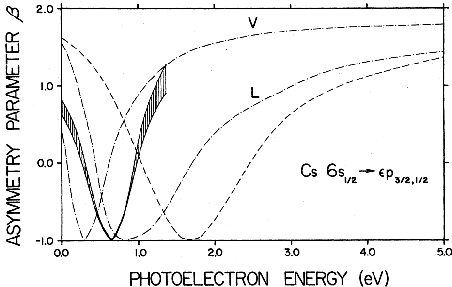
FIG. 4. Angular distribution asymmetry parameter \beta(E) vs photoelectron energy (eV); -·-, present frozen-core results in dipole-length ( L ) and dipole-velocity ( V ) approximation; shaded band, inferred experimental results obtained from data of Baum et al. (Ref. 9) for X(E) ; ---, Dirac-Fock calculation of Ong and Manson (Ref. 20).
