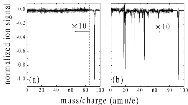
FIG. 2. Mass spectra of toluene. Panel (a): 300-mm focal length lens; I_w = 7 \times 10^{10} \text{ W cm}^{-2} , I_f = 1 \times 10^{14} \text{ W cm}^{-2} ; panel (b): 1000-mm focal length lens; I_w = 3 \times 10^{11} \text{ W cm}^{-2} , I_f = 6 \times 10^{13} \text{ W cm}^{-2} .
