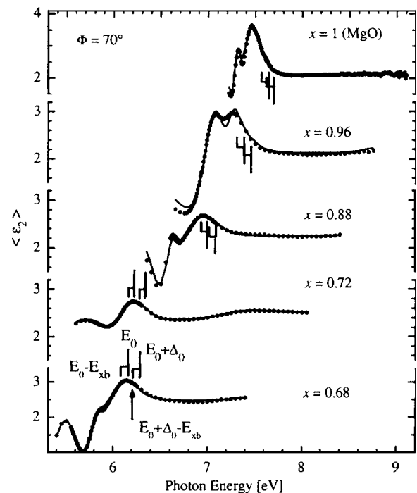
FIG. 4. Experimental (symbols) and best-model calculated (CP-MDF: solid lines) \langle \epsilon_2 \rangle spectra for various \text{Mg}_x\text{Zn}_{1-x}\text{O} films deposited on c -plane sapphire. Brackets with vertical bars indicate the transition energies E_0 and E_0 + \Delta_0 (long bar), and their respective exciton resonance E_0 - E_{xb} and E_0 + \Delta_0 - E_{xb} (short bar).
