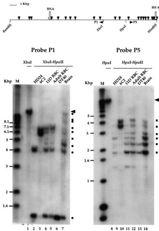
Fig. 10. Establishment of a fully methylated region between the folate receptor gene and the \beta -globin locus at the CFU-E stage. The map shows the position of XbaI and HpaI restriction sites and probes P1 and P5 used to look for HpaII cutting. Small arrows represent HpaII sites. Analysis of HpaII methylation toward the folate receptor gene is shown on the left panel. Genomic DNA from different tissues or cell lines was digested with XbaI + HpaII and detected with probe P1. The small arrow indicates the parental band. Dots show the position of HpaII sites. Analysis of HpaII methylation toward the insulator is shown on the right panel. Genomic DNA from different tissues or cell lines was digested with HpaI + HpaII and detected with probe P5. The small arrow indicates the parental band.
