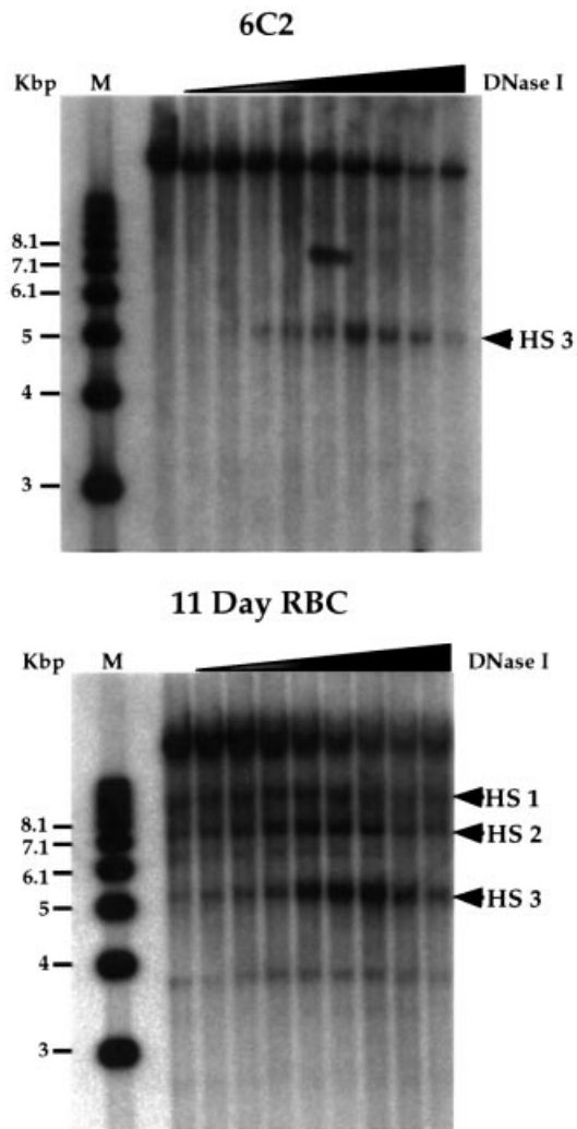
Fig. 8. Detection of DNase I hypersensitive sites. DNA from DNase I-treated nuclei (6C2 cells or 11 Day RBC) was digested with KpnI and probed with probe P6. The hypersensitive bands corresponding to HS1, HS2 and HS3 are indicated.
