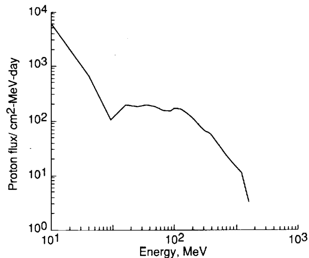
Figure 7. Trapped proton energy spectrum for STS-42.
