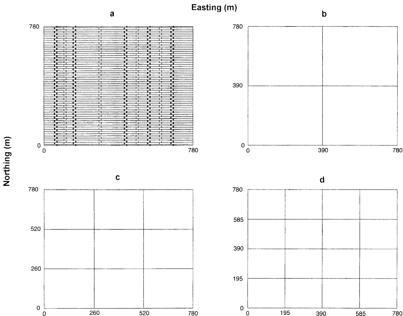
Fig. 1. The grid arrangements for the multifractal analysis. (a) is the sampling grids of the soil NO 3 -N and grain yield for the uniform N treatment (sampling point is indicated by a dot); (b), (c), and (d) are different multifractal cell sizes.
