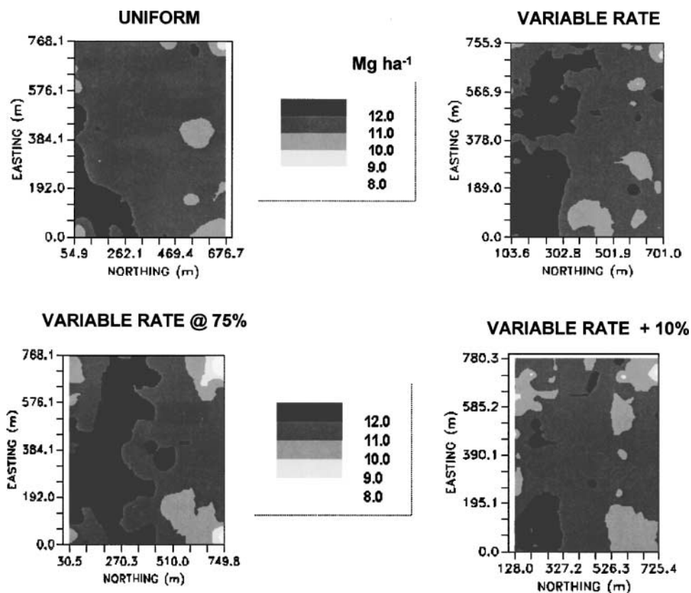
Fig. 7. Corn grain yield distribution for four treatments in 1997. Each map was generated using the data from the strips of that treatment.
