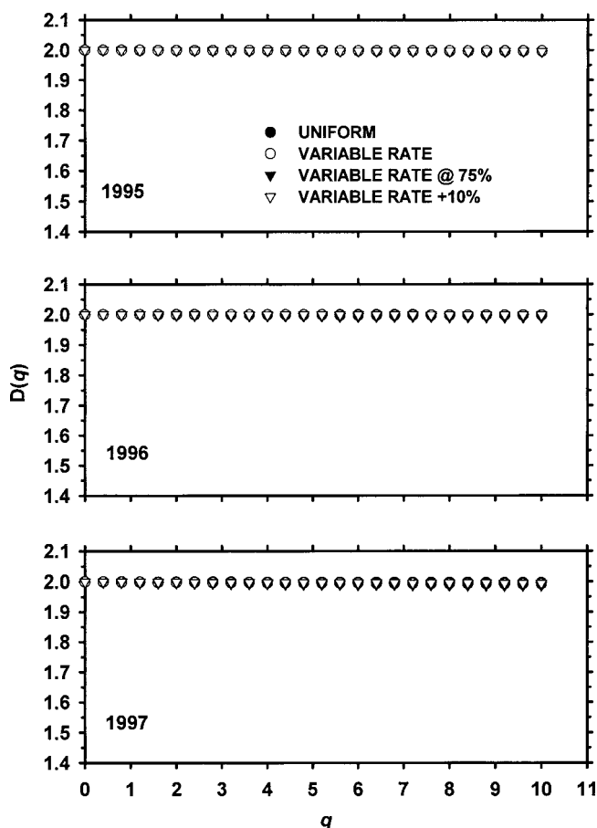
Fig. 5. Corn grain yield D(q) values as a function of increasing q values for four N treatments in 3 yr.
