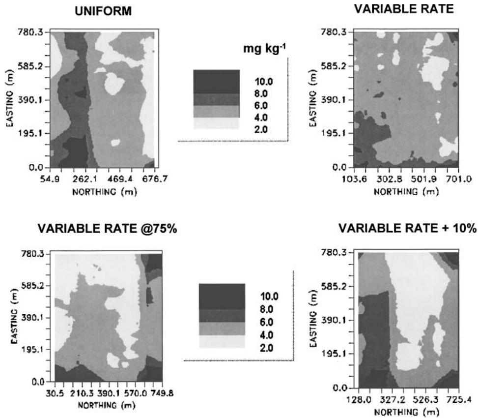
Fig. 4. Residual soil NO 3 -N distribution for four treatments in 1995. Each map was generated using the data from the strips of that treatment.
