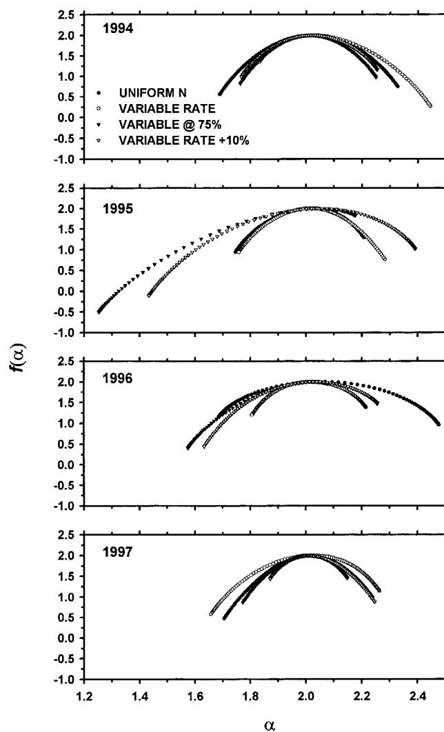
Fig. 3. Multifractal spectrums for residual soil \text{NO}_3\text{-N} for four N treatments in 4 yr.
