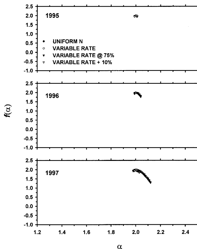
Fig. 6. Multifractal spectrums for corn grain yield for four N treatments in 3 yr.
