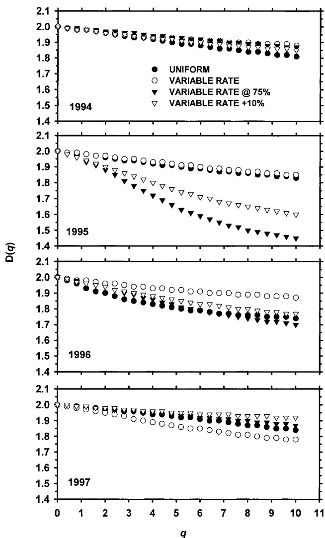
Fig. 2. Residual soil nitrate D(q) values as a function of increasing q values for four N treatments in 4 yr.
