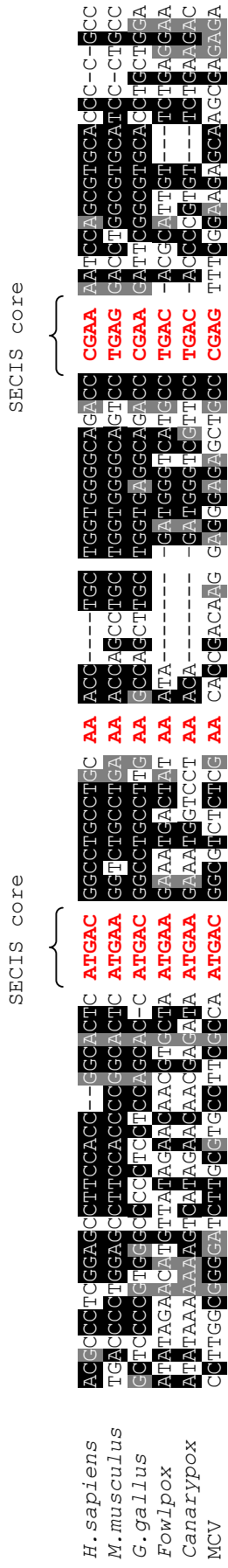
Figure S2. Alignment of GPx4 SECIS elements.
