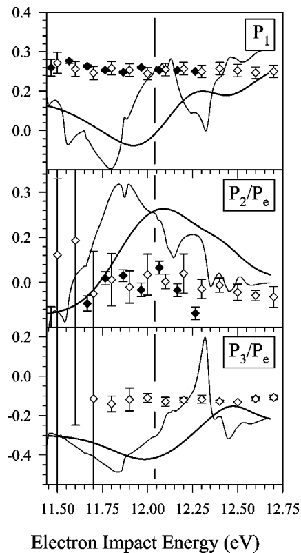
FIG. 6. Integrated Stokes parameters for the 878 nm transition in Kr ( 4p^5 5p[5/2] \ ^3D_2 \rightarrow 4p^5 5s[3/2] \ ^3P_1 ). The vertical line at 12.04 eV represents the cascade threshold. All other designations are as in Fig. 5.
