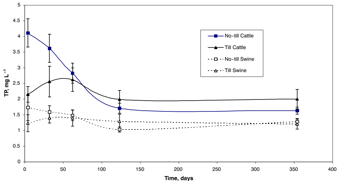
Figure 2c. Total phosphorus (TP) concentrations of runoff versus time since manure application for the experimental treatments. Vertical bars represent one standard deviation of the mean value.
