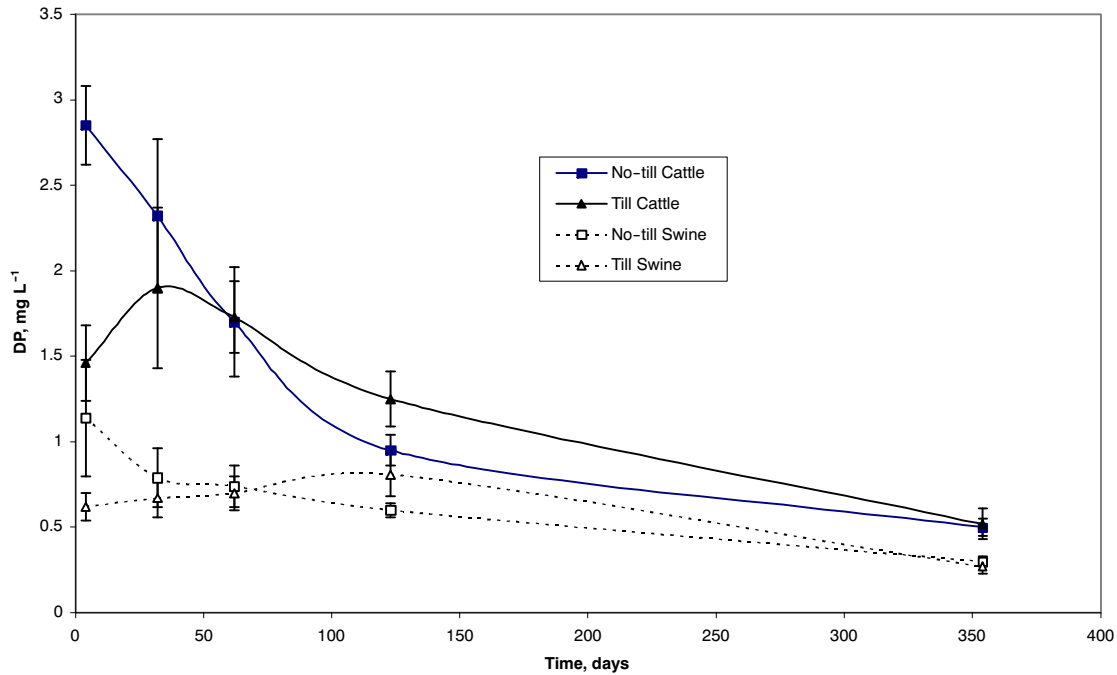
Figure 2a. Dissolved phosphorus (DP) concentrations of runoff versus time since manure application for the experimental treatments. Vertical bars represent one standard deviation of the mean value.
