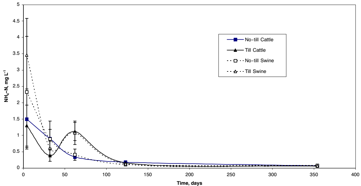
Figure 3b. \text{NH}_4\text{-N} concentrations of runoff versus time since manure application for the experimental treatments. Vertical bars represent one standard deviation of the mean value.
