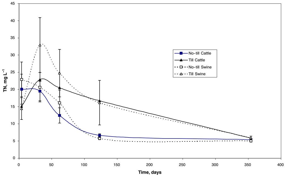
Figure 3c. Total nitrogen (TN) concentrations of runoff versus time since manure application for the experimental treatments. Vertical bars represent one standard deviation of the mean value.
