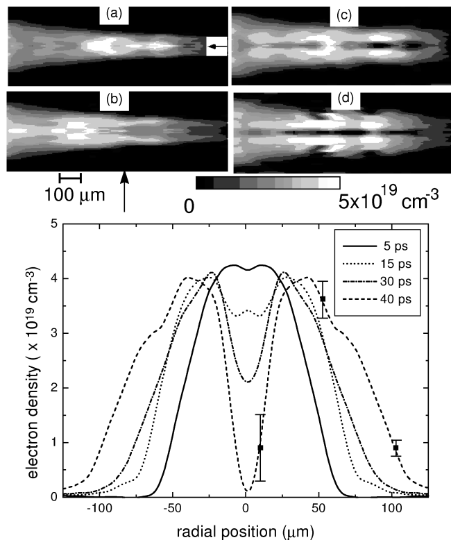
FIG. 3. 3D plasma density distribution for 2.5-TW laser power and 2 \times 10^{19} -cm ^{-3} gas density at different times: (a) 5 ps, (b) 15 ps, (c) 30 ps, and (d) 40 ps. Lineouts of the cross sections at the position indicated by the vertical arrow are shown along with the error bars at three selected positions.
