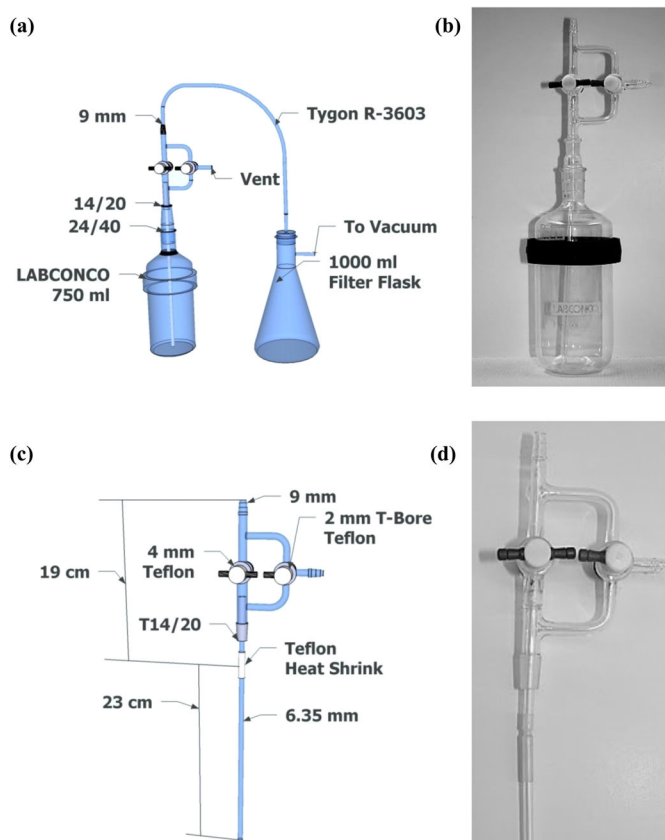
Figure 1. Schematic drawing (a) and picture (b) of our NMR tube cleaning apparatus. Schematic drawing (c) and picture (d) of an expanded view of the glass switch. Important features and dimensions are labeled.
