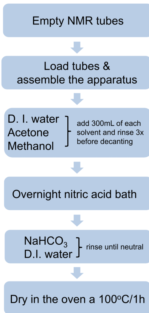
Figure 2. Flow diagram of the NMR tube cleaning process.
