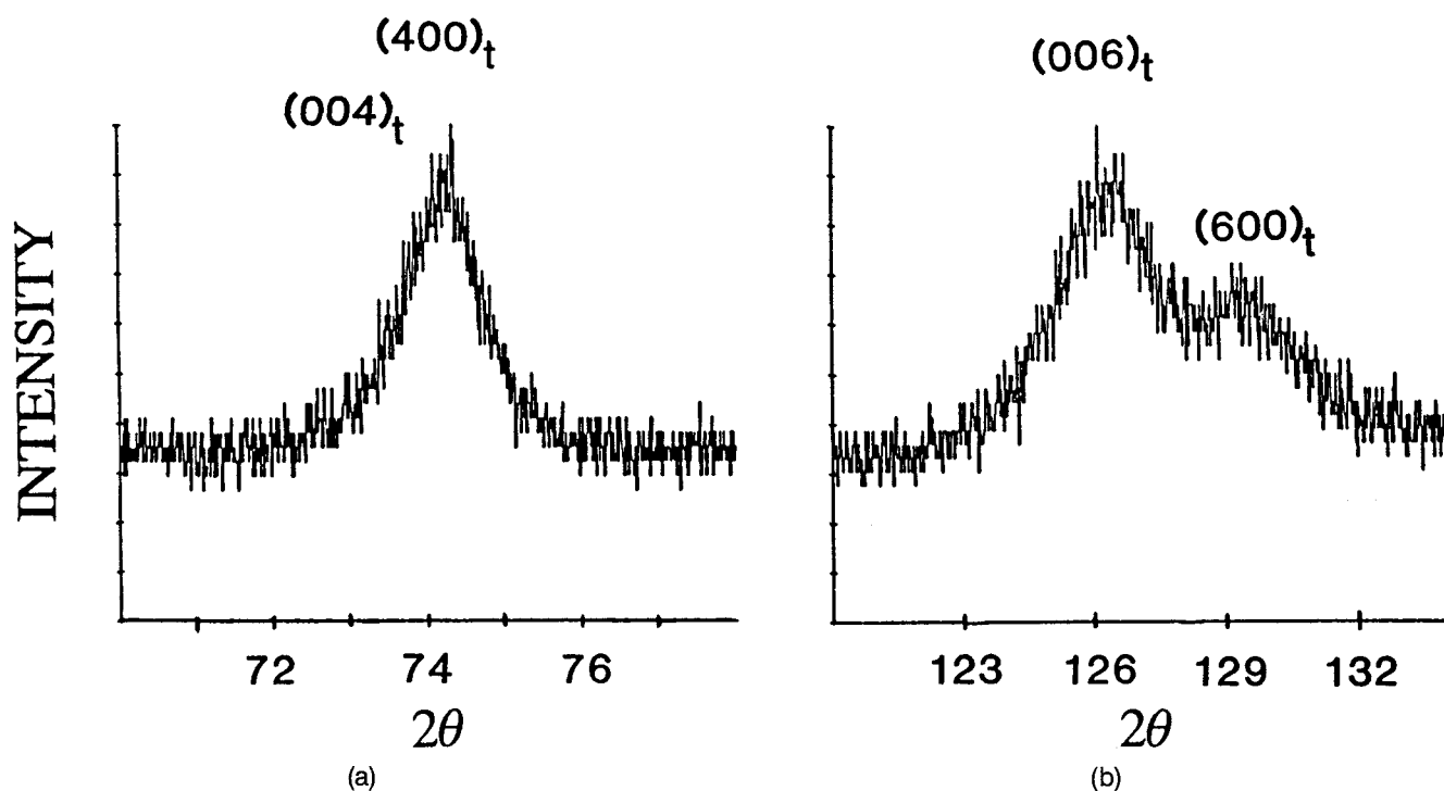
FIG. 4. X-ray diffraction patterns for sample D. Although the (004)_t and (400)_t are not well resolved, the (006)_t and (600)_t profiles can be seen clearly resolved.
