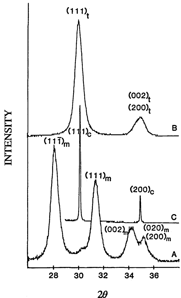
FIG. 1. Typical x-ray diffraction patterns using a synchrotron source. (A) 100% monoclinic zirconia precipitated at pH 10.5 and calcined at 500 °C–5 h, (B) 100% tetragonal zirconia (sample C) and (C) 100% cubic zirconia (sample A).
