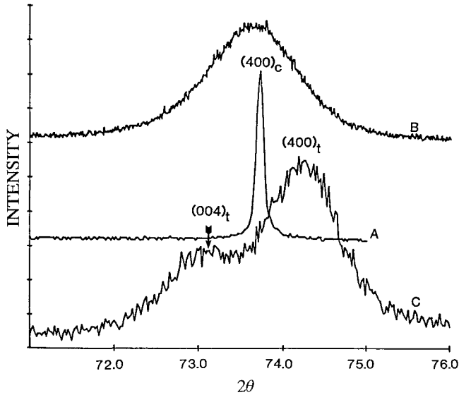
FIG. 2. X-ray diffraction pattern for samples A, B, and C in the 2\theta region of 71\text{--}76^\circ , where the (400) cubic peak and (004) (400) tetragonal doublets should appear. Curves (A), (B), and (C) refer to samples A, B, and C, respectively.
