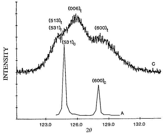
FIG. 3. X-ray diffraction patterns for samples A and C in the 2\theta region of 120\text{--}134^\circ . Sample A shows (531) and (600) cubic peaks. Sample C shows the overlapping (513) and (531) tetragonal doublets. The (006) and (600) tetragonal doublet can be observed clearly without overlap.
