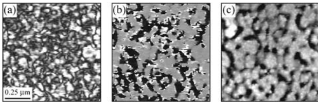
FIG. 2. LPFM (a) amplitude and (b) phase of a 1 \times 1 \mu\text{m}^2 region of a tetragonal (111) PZT thin film and the corresponding (c) topography.
