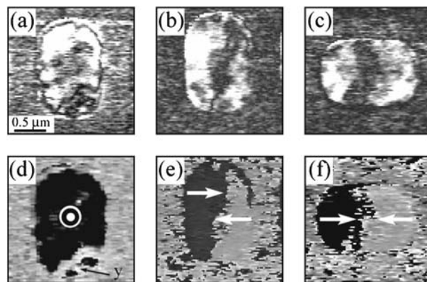
FIG. 5. VPFM and LPFM images of (a, b) amplitude and (d, e) phase, respectively, of a ferroelectric capacitor with nonuniform out-of-plane polarization. LPFM (c) amplitude and (f) phase of the same capacitor following a 90° clockwise rotation of the sample. The presence of adjacent positive and negative domains in the region marked “y” and also along the edge of the capacitor suggests the existence of 180° domain walls. However, the possibility of non-through domains makes an exact determination of the domain wall type difficult.
