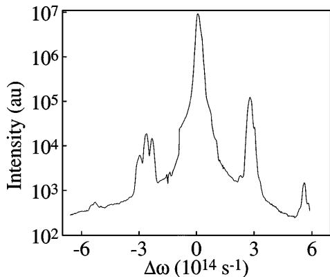
FIG. 1. Spectrum of the Thomson scattered probe light for a helium backing pressure of 100 psi, P_{\text{pump}} = 3 TW, and \Delta t = 0 .
