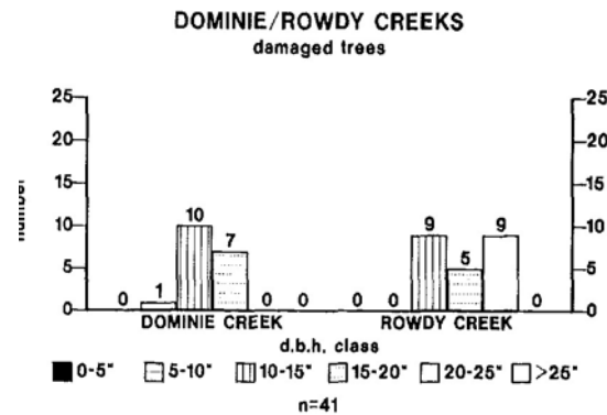
Figure 3. Distribution and size of redwoods that sustained feeding injuries at both Rowdy Creek and Dominie Creek sites.
