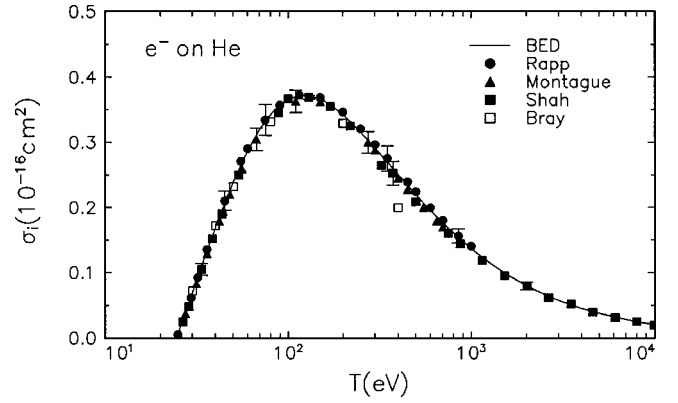
FIG. 1. Total cross section for ionization of He by electron impact. The abscissa is the incident electron energy T in eV. Solid line, BED cross section; filled circles, experimental data by Rapp and Englander-Golden [3]; filled triangles, data by Montague et al. [4]; filled squares, data by Shah et al. [1]; open squares, CCC theory by Fursa and Bray [8].
