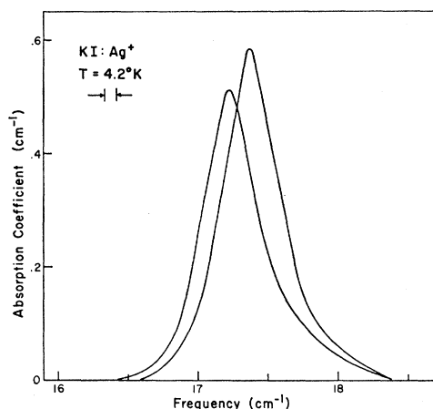
FIG. 3. Impurity-induced absorption coefficient versus frequency for ^{107}\text{Ag}^+ and ^{109}\text{Ag}^+ impurities in KI. No \text{Ag}^+ concentrations are given because of the uncertainty about what fraction of the \text{Ag}^+ ions are actually participating in the resonant mode. (See Sec. II B of this paper.) The interferometer resolution is indicated by the separation of the two arrows.
