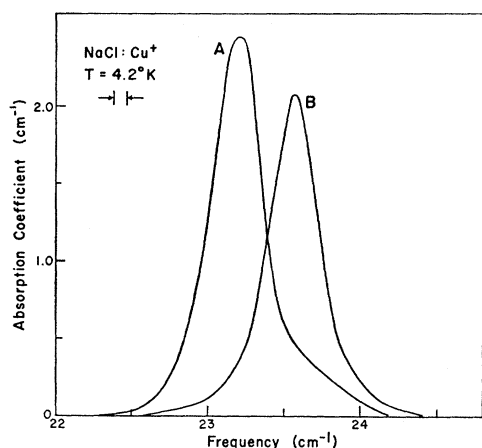
FIG. 1. Impurity-induced absorption coefficient versus frequency for ^{63}\text{Cu}^+ and ^{65}\text{Cu}^+ impurities in NaCl. Curve A has 1.15 \times 10^{17} ( ^{63}\text{Cu}^+ ions)/ \text{cm}^3 , and curve B has 1.06 \times 10^{17} ( ^{65}\text{Cu}^+ ions)/ \text{cm}^3 . The interferometer resolution is indicated by the separation of the two arrows.
