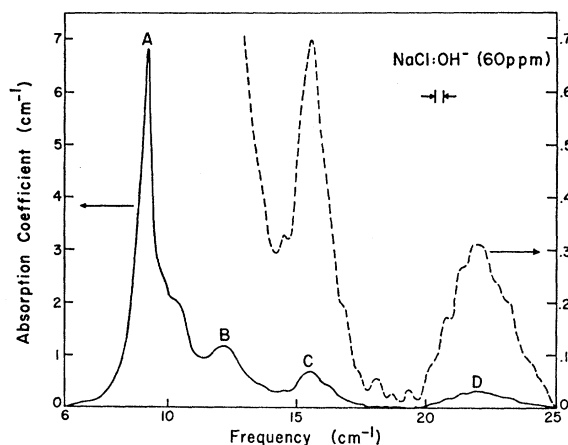
FIG. 2. Impurity-induced absorption coefficient versus frequency for NaCl: \text{OH}^- . Note the factor-of-10 change in the absorption coefficient scale for the dotted curve. The small "wiggles" on the dotted curve are instrumental. Line A is at 9.2 \text{ cm}^{-1} , line B is at 12.2 \text{ cm}^{-1} , line C is at 15.6 \text{ cm}^{-1} , and line D is at 22.0 \text{ cm}^{-1} . The interferometer resolution is indicated by the separation of the two arrows. The sample temperature was 4.2^\circ\text{K} .
