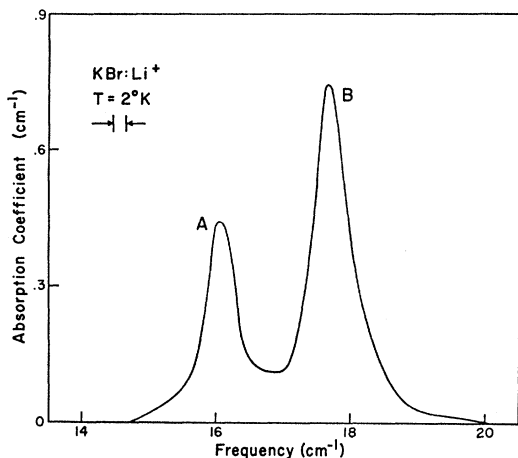
FIG. 5. Impurity-induced absorption coefficient versus frequency for {}^6\text{Li}^+ and {}^7\text{Li}^+ impurities in KBr. Peak A corresponds to 1.9 \times 10^{16} ( {}^7\text{Li}^+ ions)/ \text{cm}^3 , and peak B corresponds to 3.7 \times 10^{18} ( {}^6\text{Li}^+ ions)/ \text{cm}^3 . The interferometer resolution is indicated by the separation of the two arrows.
