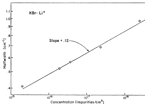
FIG. 6. Concentration dependence of the full width at half-maximum absorption for KBr: \text{Li}^+ . The experimental widths have been corrected for the instrumental width, assuming a Gaussian absorption line and slit function. Note the log-log coordinates.
