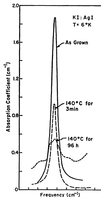
FIG. 4. Temperature instability of the silver-activated resonant-mode in KI. The far-infrared transmission was measured with the crystal at 6^\circ\text{K} between each cycle to 413^\circ\text{K} . For this low-resolution study, the line shape is determined by the instrumental width of 1\text{ cm}^{-1} .
