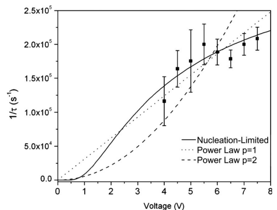
FIG. 6. Reciprocal switching time as a function of applied voltage recorded at 25 °C with a nanomesa sample made from a 3-ML copolymer LB film and 3-ML insulating PSMA film. The voltage pulses were 400 \mu s in duration.
