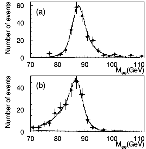
FIG. 6. Dielectron mass distributions for (a) edge electrons with E_T > 41 GeV and (b) edge electrons with E_T < 41 GeV. The histograms are the best fit distributions from the Monte Carlo. The curve at the bottom of (b) represents the background.
