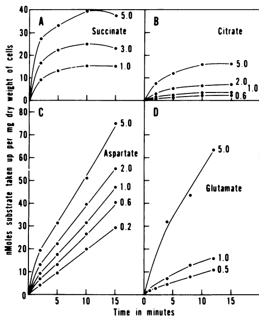
FIG. 1. Kinetics of substrate uptake by B. thuringiensis var. entomocidus . Substrate concentrations shown in mM: (A) [2,3-^{14}\text{C}] succinate; (B) [1,5-^{14}\text{C}] citrate; (C) [U-^{14}\text{C}] aspartate; (D) [3,4-^{14}\text{C}] glutamate. Final cell concentration was 1.0 mg (dry weight)/ml for A, B, and C, and 0.1 mg (dry weight)/ml for D.
