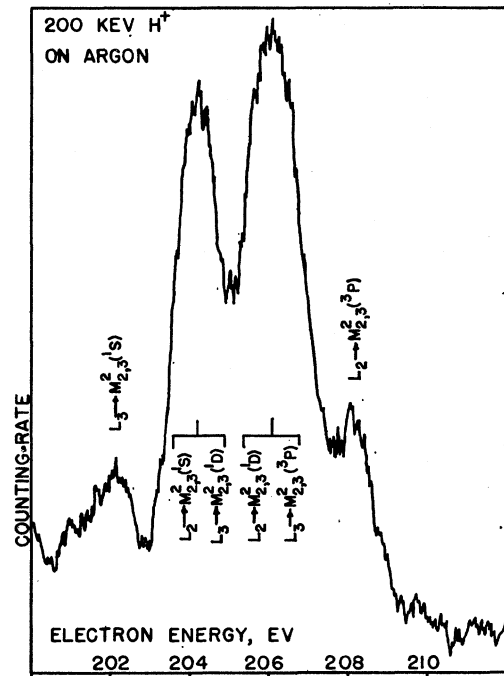
FIG. 5. Energy spectrum of electrons from 200-keV H^+ -Ar collisions. Resolution about 1.4 eV.
