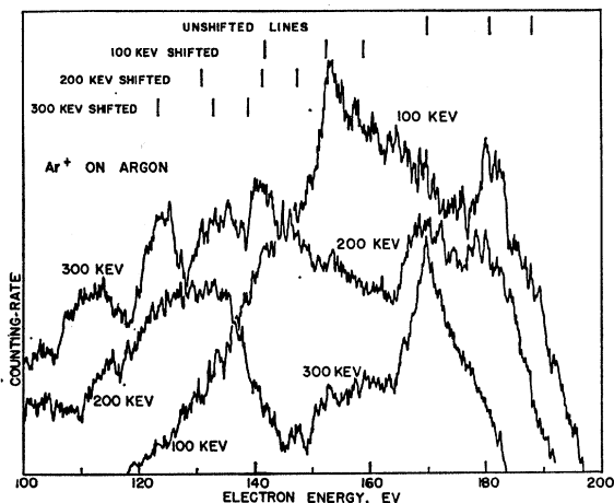
FIG. 3. Energy spectrum of electrons from \text{Ar}^+ -Ar collisions. Resolution about 3 eV.
