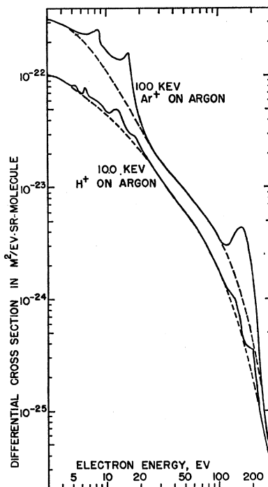
FIG. 1. Doubly-differential cross-sections for ejection of electrons from argon by protons and argon ions at 100 keV. Electrons are detected at 160^\circ from the beam direction. Resolution varies from 0.5 eV at 3 eV energy to 12 eV at 300 eV.
