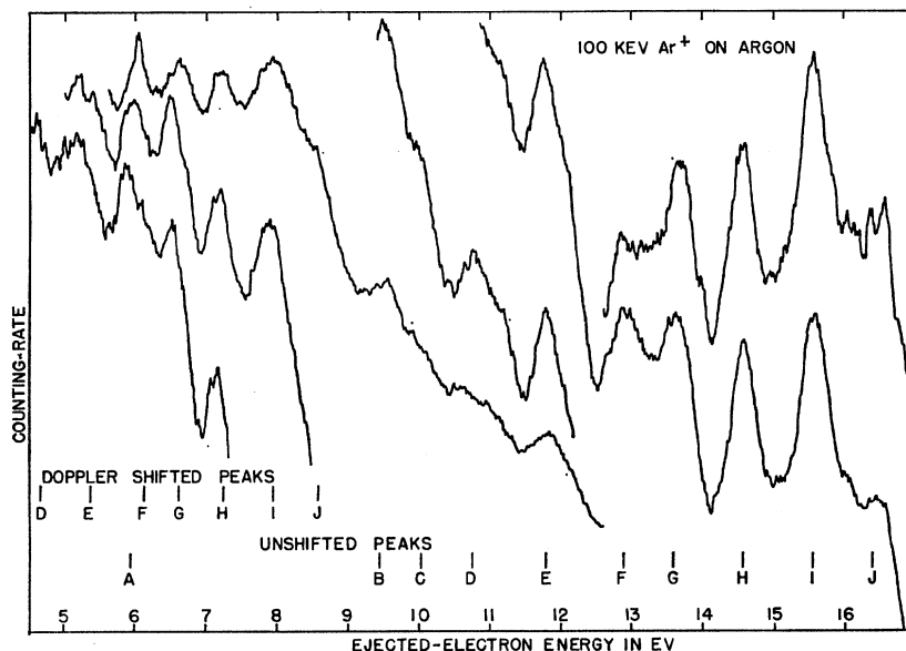
FIG. 2. Energy spectrum of electrons from 100-keV \text{Ar}^+ -Ar collisions. Resolution about 0.2 eV.
