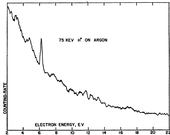
FIG. 4. Energy spectrum of electrons from 75-keV H^+ -Ar collisions. Resolution about 0.2 eV.
