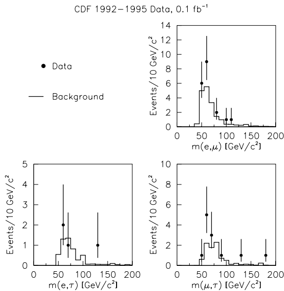
FIG. 2. The reconstructed mass of the lepton pairs. The points show the nineteen e\mu candidates (upper), the four e\tau candidates (lower left), and the twelve \mu\tau candidates (lower right). The histograms show the total background in each sample. The e\tau and \mu\tau samples have no events in common; both are subsets of the e\mu sample. \cancel{E}_T is used in computing \tau momentum, as explained in the text.
