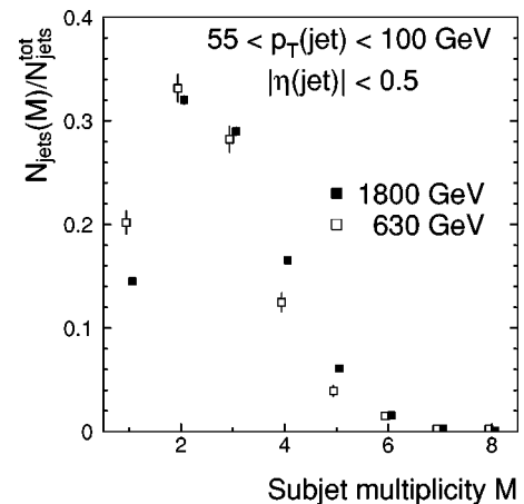
FIG. 18. Uncorrected subjet multiplicity in jets from D\bar{D} data at \sqrt{s}=1800 GeV and 630 GeV.
