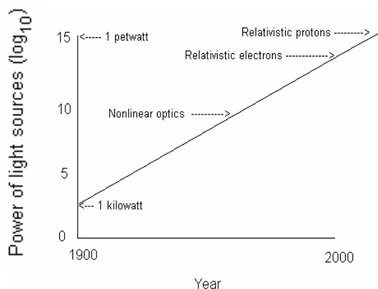
Figure 1 As the power of laboratory light sources increases the energy of accelerated particles increases accordingly, making laser-induced nuclear reactions possible. The most powerful lasers have now reached petawatt ( 10^{15} watts) peak powers, allowing them to accelerate electrons to relativistic speeds. The gamma rays produced by such electrons have been used in recent experiments to split the uranium atom 3,4 .
