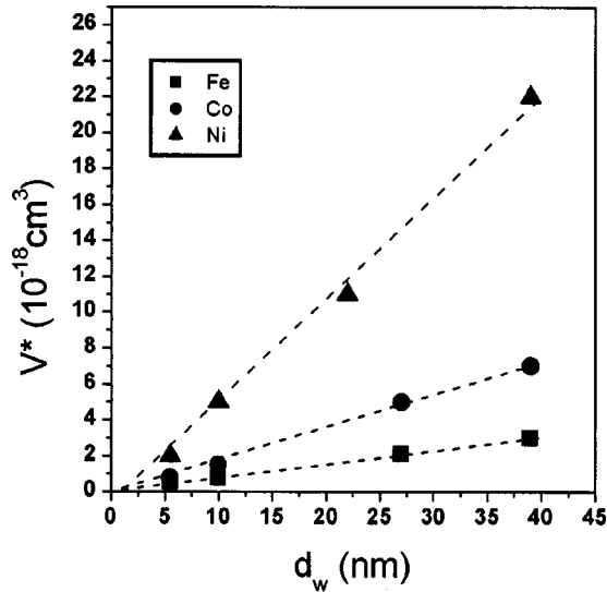
FIG. 3. V^* as a function of d_w for Fe, Co, and Ni nanowires, respectively. The dashed lines are guides to the eye.
