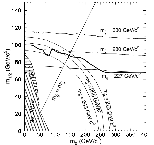
FIG. 2. Exclusion contour in the (m_0, m_{1/2}) plane for \tan\beta = 2 , \mu < 0 , A_0 = 0 , and finite \lambda'_{2jk} ( j = 1, 2; k = 1, 2, 3 ) coupling. The region below the bold line is excluded at the 95% C.L. The crosshatched region is excluded for theoretical reasons (see text). m_{\tilde{q}} and m_{\tilde{g}} denote squark and gluino masses, respectively.
