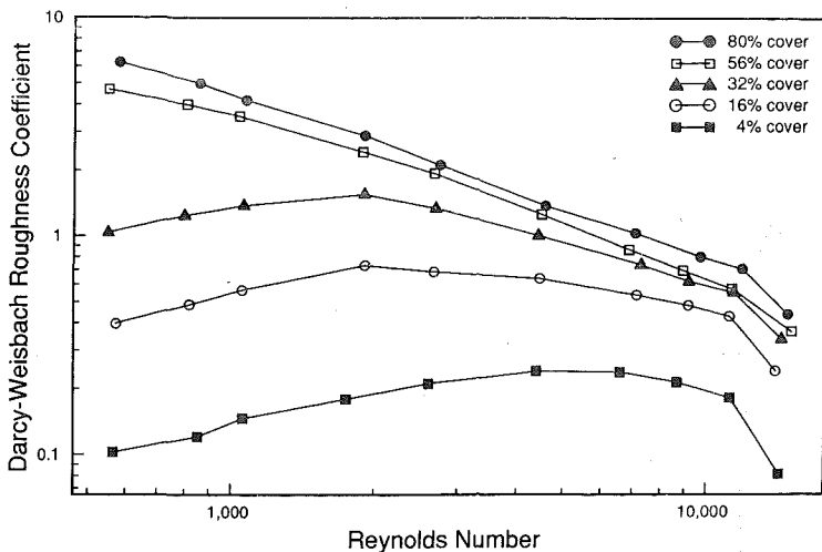
FIG. 1. Darcy-Weisbach Roughness Coefficients versus Reynolds Number for Gravel Material with 2.54–3.81-cm Diameter
