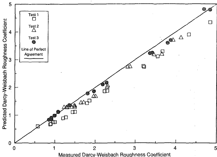
FIG. 3. Predicted versus Measured Darcy-Weisbach Roughness Coefficients
