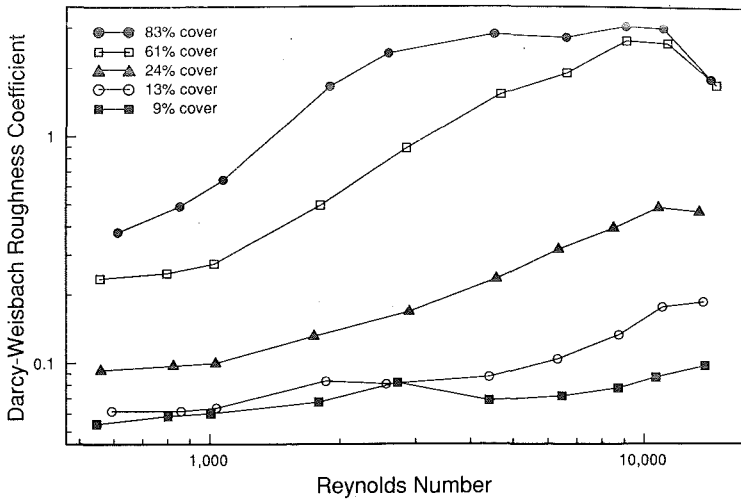
FIG. 2. Darcy-Weisbach Roughness Coefficients versus Reynolds Number for Cobble Material with 12.70–25.40-cm Diameter
