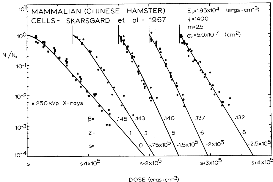
FIG. 7. Chinese hamster cells. Survival data from Skarsgard et al. [6] are superimposed on fitted survival curves. Data obtained with 250-kVp X-rays are compared to a curve calculated for 10-MeV protons.
