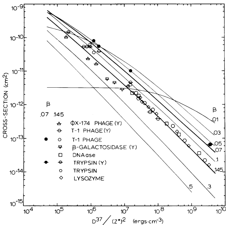
FIG. 3. Cross-section for the inactivation of dry enzymes and viruses divided by the square of the effective charge number of the bombarding ion. Plotted points crossed with a horizontal bar were obtained at the Yale HILAC (Y), while other points were obtained at the Berkeley HILAC. Lines arise from the theory [1].
