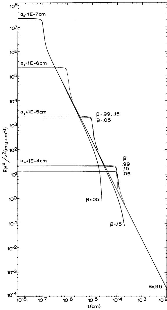
FIG. 1. The mean dose \bar{E} deposited by secondary electrons in a short cylinder of radius a_0 , whose axis is parallel to and t distant from the path of an ion of effective charge ze , moving at relative speed \beta , for a range of values of a_0 . In water.
