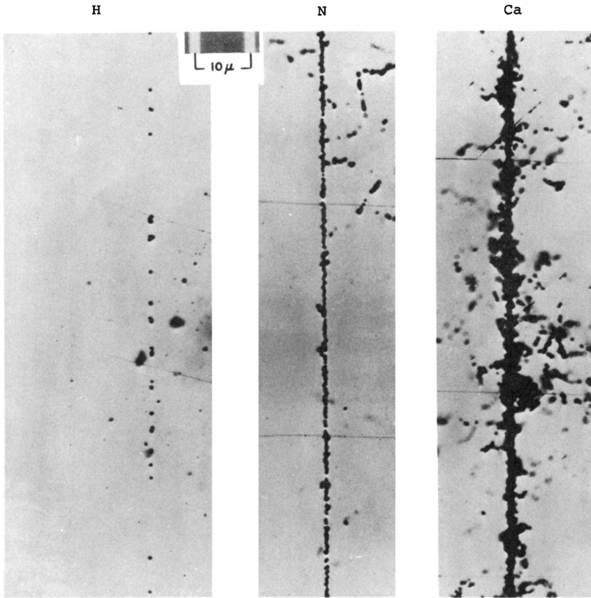
FIG. 2. Tracks of relativistic protons, nitrogen and calcium nuclei in Ilford G.5 emulsion illustrate the grain count and track width regimes, and the transition between them. Courtesy M. M. Shapiro, Naval Research Laboratory.
