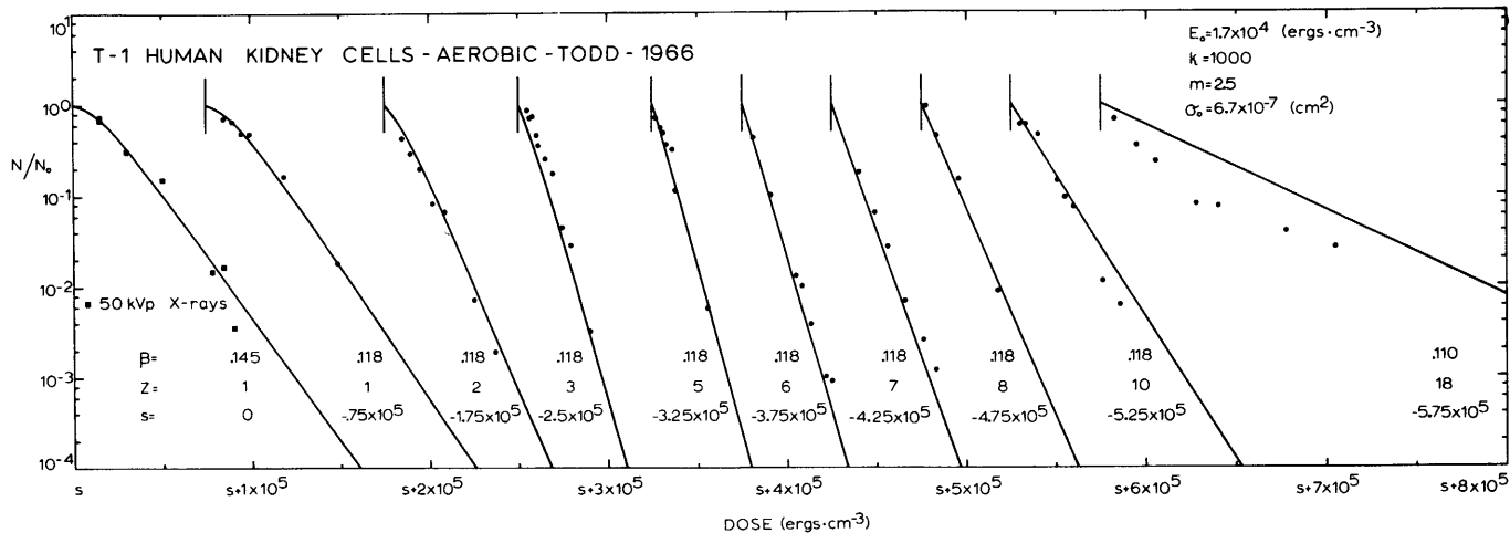
FIG. 6. T-1 human kidney cells - aerobic. Survival data from Todd [8] are superimposed on fitted survival curves for given z and \beta , nested by use of a horizontal displacement parameter s . Data obtained with 50-kVp X-rays are compared to calculations for 10-MeV protons. The departure of the data from the curve for Z = 18 is evidence that kidney cells are in the trackwidth regime at this bombardment.
