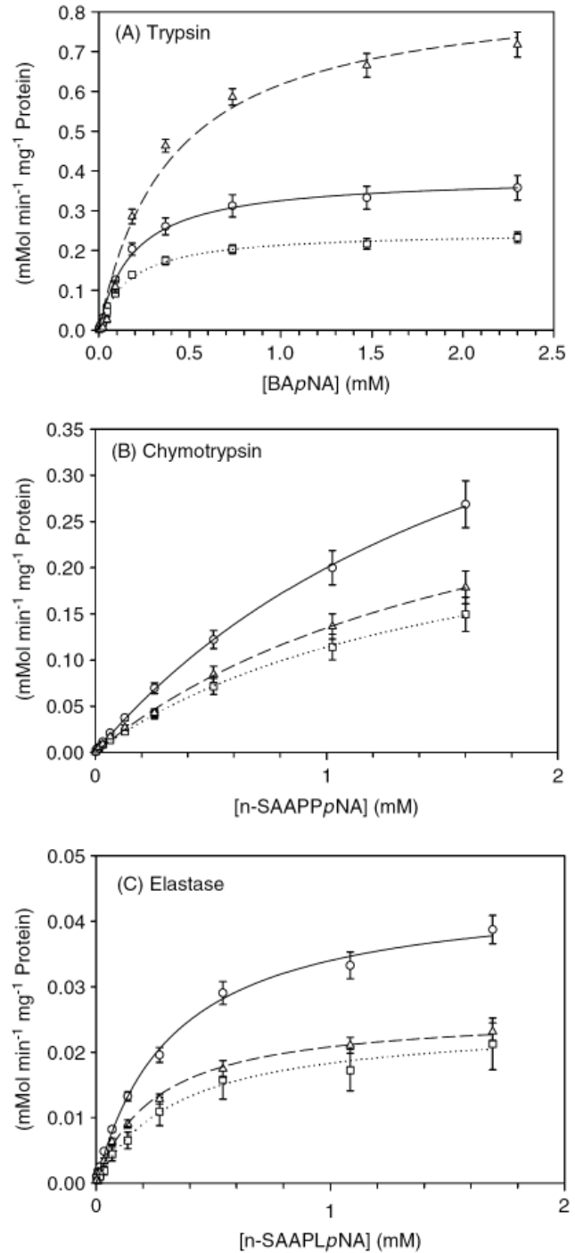
Figure 2. Specific activities of (A) trypsin-like, (B) chymotrypsin-like and (C) elastase-like proteinases from (○) Europe-S, (□) Europe-R, and (Δ) RSTT-R at 10 concentrations of substrate. Each curve represents an average of three different preparations (three replicates per sample). Bars represent the standard errors of the means (SEM). Non-linear regressions were significant at P < 0.001 .
