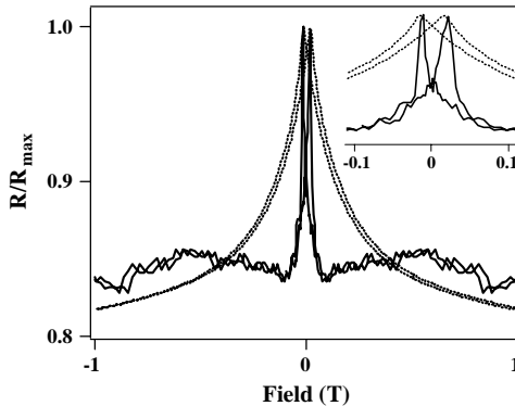
Fig. 1 – Magnetoresistance curve at 3K of a chromium oxide thin film with an electric percolation path through a few (typically 10) CrO 2 crystallites. The dotted curve is a measurement performed on a low-resistance chromium oxide thick film, where the percolation path goes through many (estimated larger than 100) crystallites.
