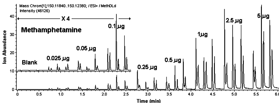
Figure 3. m/z 150 ion chromatogram for triplicate IPA-soaked wipe samples for no methamphetamine and eight levels of methamphetamine deposited on 10 \times 10 -cm mirror squares.
