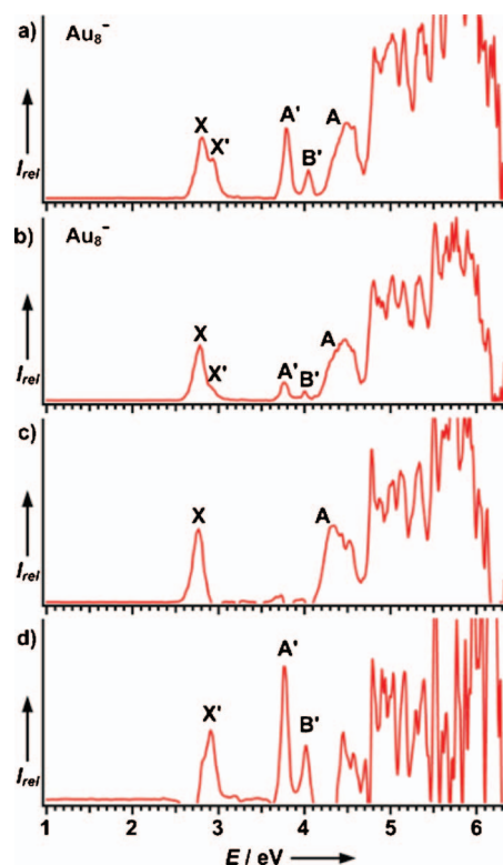
FIG. 3. Photoelectron spectra of \text{Au}_8^- . (a) Using pure He carrier gas; (b) using a 5% \text{O}_2/\text{He} reactant gas with the flow tube reactor; (c) the spectrum of the D_{4h} isomer obtained by subtracting (d) from (b); and (d) the spectrum of the C_{2v} isomer obtained by subtracting (b) from (a).
