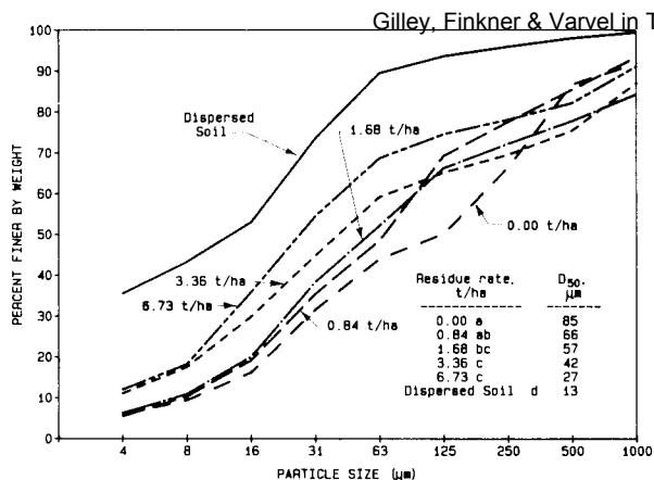
Fig. 1—Size distributions of eroded sediment for five sorghum residue treatments and dispersed soil. For the residue rates listed in the lower right table, differences in size distributions of sediment are significant at the 5% level (Pearson chi-square test) if the same letter does not appear.
