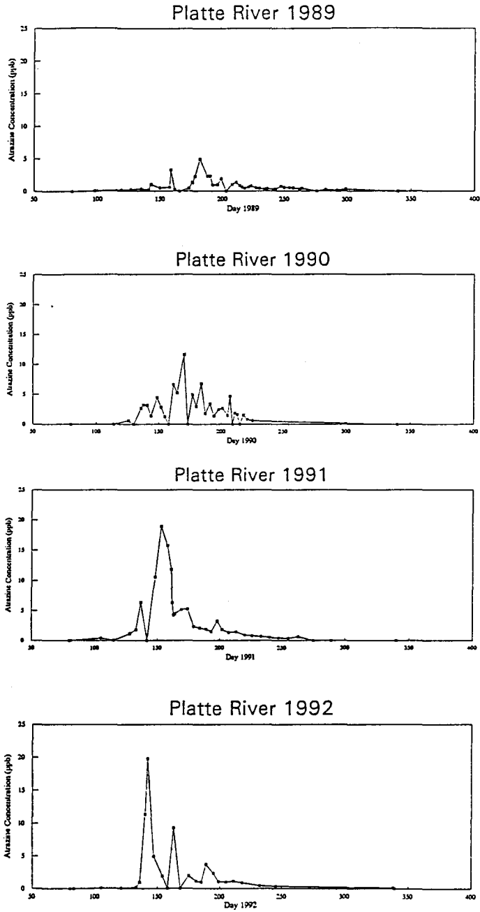
Figure 3. Atrazine concentration in the Platte River in 1989, 1990, 1991, and 1992. Compilation of (Blum 1993) and (Duncan 1991).
