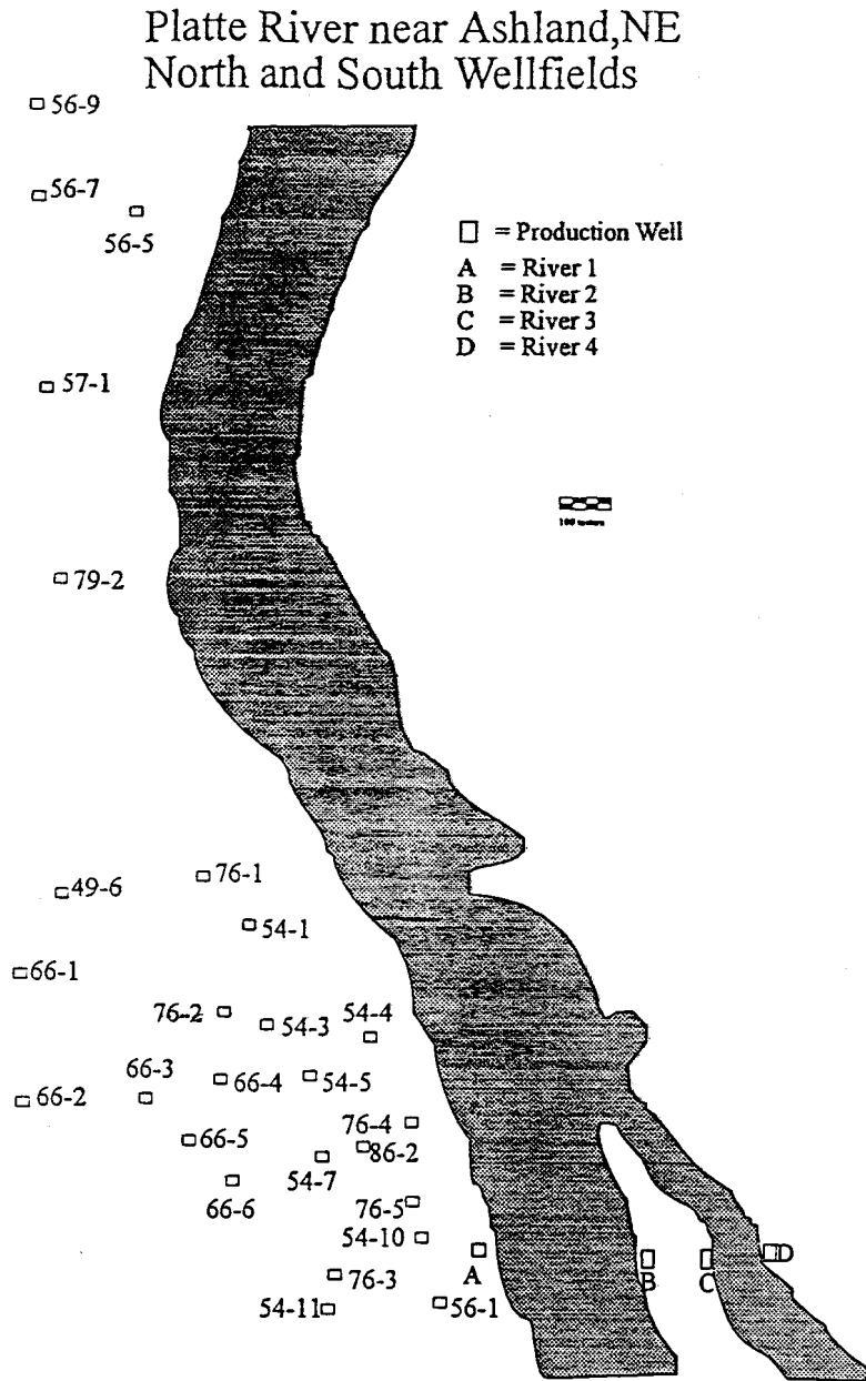
Figure 6. Map of production wells and sites for river homogeneity study.
