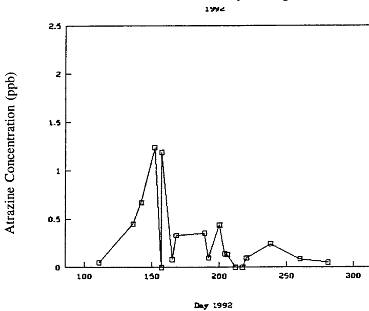
Figure 8. Concentration of atrazine in rainfall during 1992.
