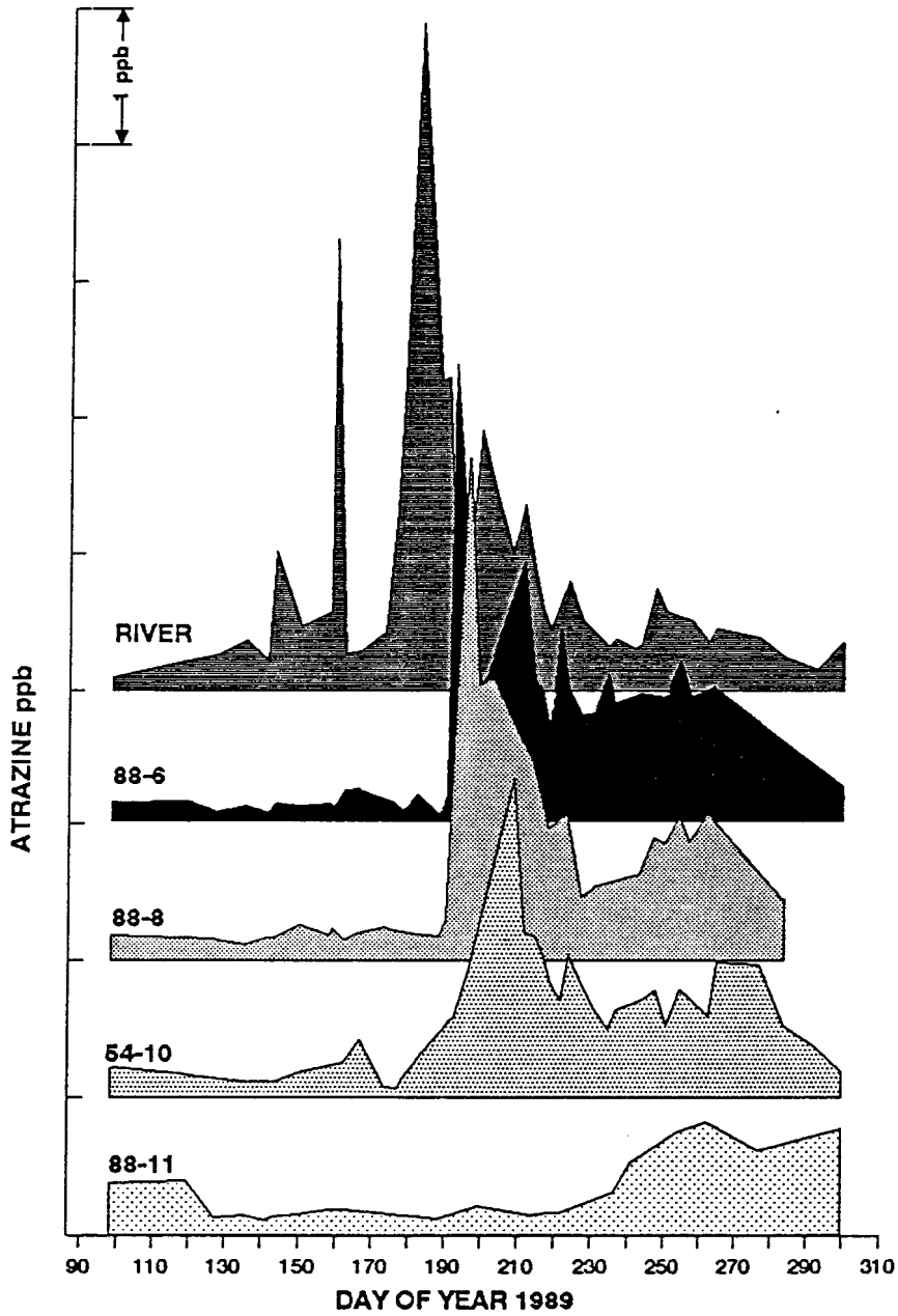
Figure 4. Concentration of atrazine in monitoring wells in the south well field in 1989 (Duncan 1991).
