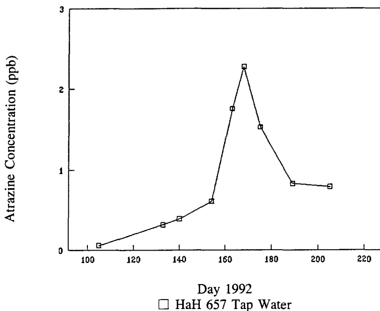
Figure 9. Concentration of atrazine in Lincoln tap water during 1992.
