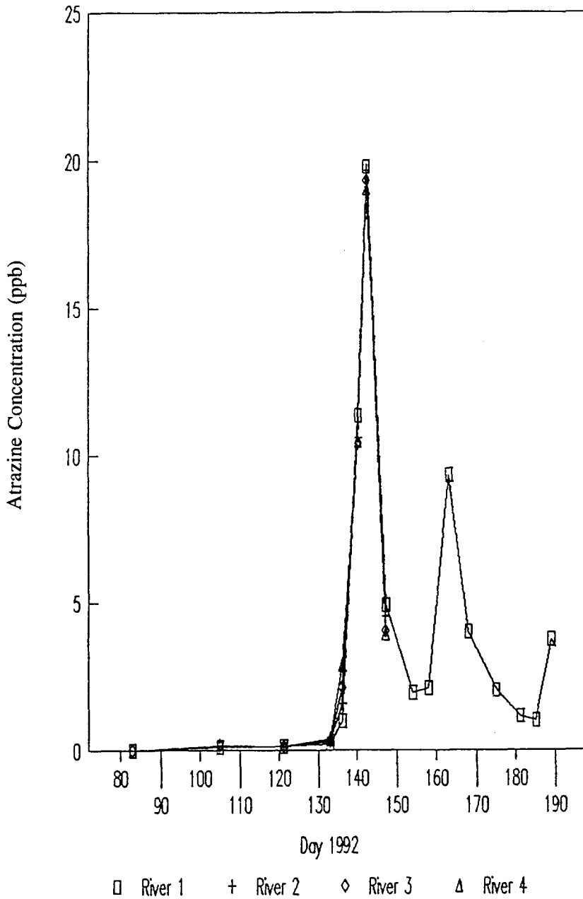
Figure 7. Concentration of atrazine in four locations of Platte River for river homogeneity study in 1992 (Blum 1992).
