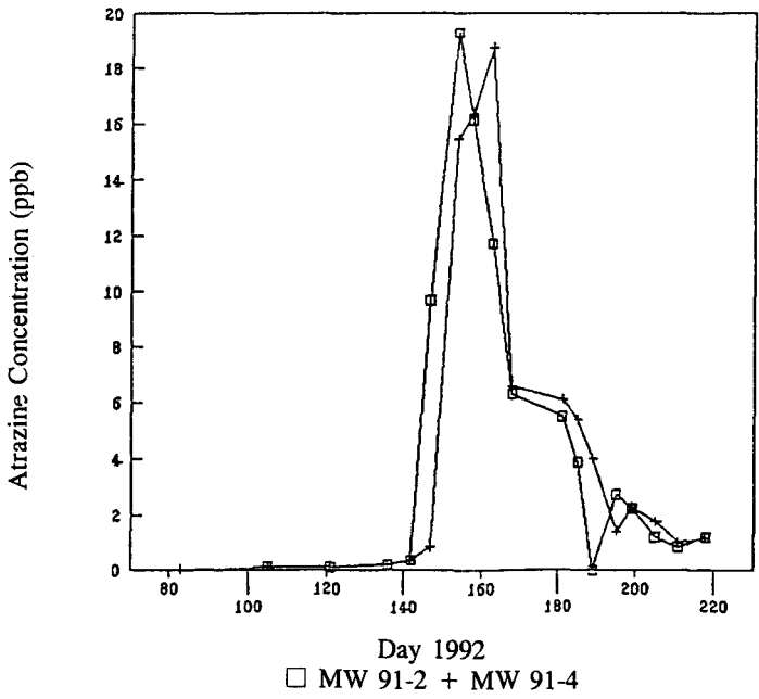
Figure 5. Concentration of atrazine in monitoring wells in the north wellfield in 1992 (Blum 1993).
