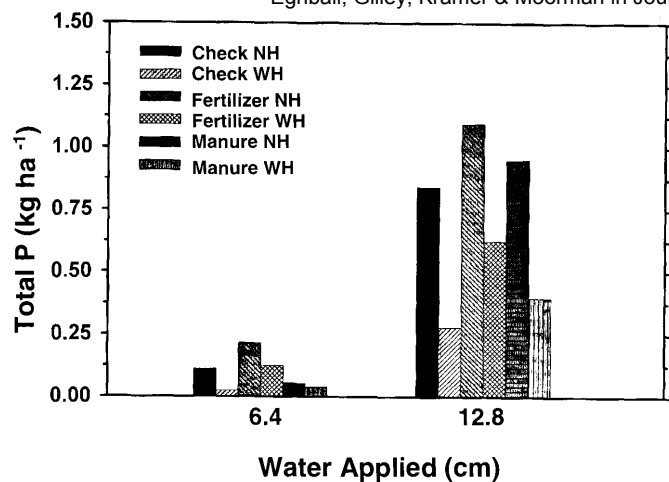
Figure 1. Total P in runoff for six treatments as influenced by water application.
