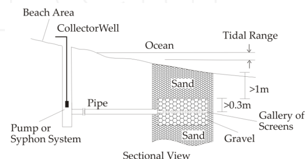
Figure 4. Seabed filtration system, adapted from [23]
