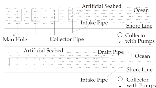
Figure 5. Alternative seabed filtration designs
