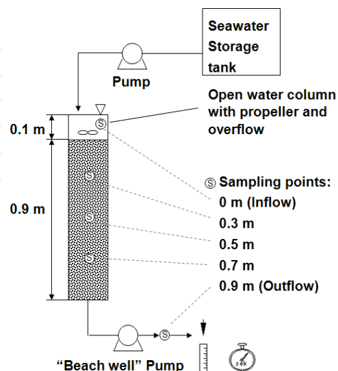
Figure 9. Experimental setup
