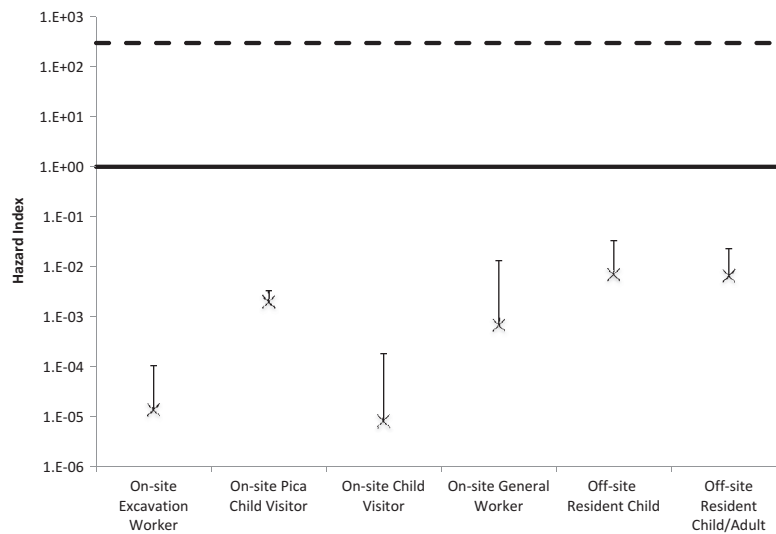
FIGURE 4. Summary of hazard index values calculated for SAN Trimer exposure scenarios. X = CTE value; error bars = RME value; solid line = exposure equivalent to the RfD value; dashed line = exposure equivalent to the BMDL value.
