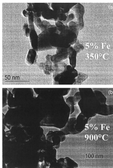
FIG. 6. Panels (a) and (b) show TEM images of \text{Sn}_{0.95}\text{Fe}_{0.05}\text{O}_2 prepared at 350 and 900^\circ\text{C} respectively.
