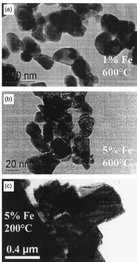
FIG. 5. Panels (a) and (b) show TEM images of \text{Sn}_{1-x}\text{Fe}_x\text{O}_2 prepared at 600^\circ\text{C} with x=0.01 and 0.05 , respectively. Panel (c) shows the TEM image of \text{Sn}_{1-x}\text{Fe}_x\text{O} prepared at 200^\circ\text{C} with x=0.05 .
