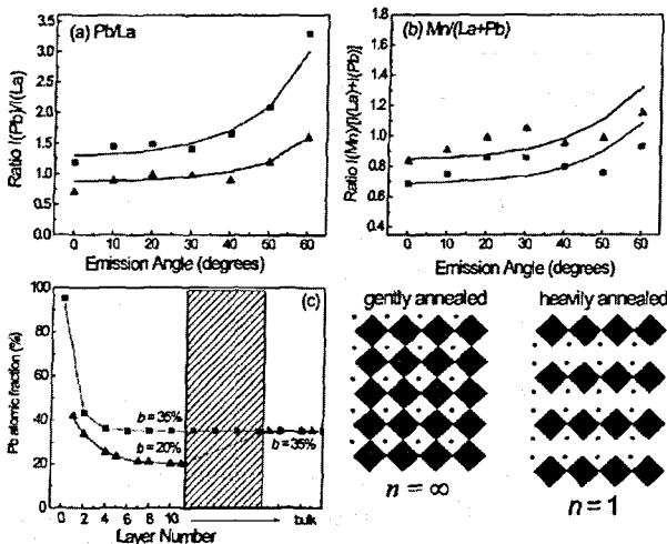
Figure 1. Panel (a) shows the normalized relative XPS core level intensity ratios of \text{Pb}(4f) peaks to that of \text{La}(3d) peaks and (b) shows the corresponding experimental and calculated intensity ratios of Mn to (\text{La}+\text{Pb}) core level intensities. The best fits (—) for the gently annealed surface ( \blacksquare ) and for the heavily annealed surface ( \blacktriangle ) of \text{La}_{0.65}\text{Pb}_{0.35}\text{MnO}_3 , as a function of photoelectron emission angle ( \theta ), are compared with the data. Panel (c) displays the resulting calculated Pb atomic fractions as a function of layer number. The inset shows schematically the layers stacking sequence used to obtain the compositional fits in panels (a) and (b) for the gently (left) and heavily (right) annealed surfaces. Adapted from [13].
