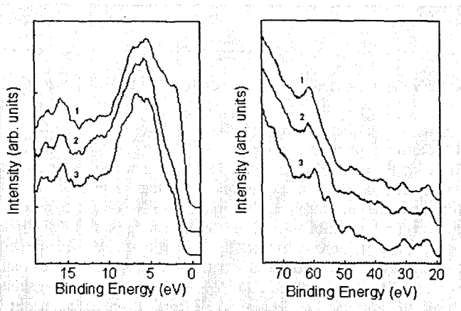
Figure 6. Photoemission spectra taken at room temperature after prolonged heating followed after several short heating/sputtering cycles: (1) prolonged annealing at 685 K, (2) after brief heating, (3) after sputtering. Spectra of the Co 3p and Fe 3p shallow cores (right panel), shows enhancement of Co 3p and/or Co and Ba Auger with annealing while the enhancement of the valence band 1.8 eV binding energy feature is shown at left. The photon energy was 115 eV. Adapted from [47].
