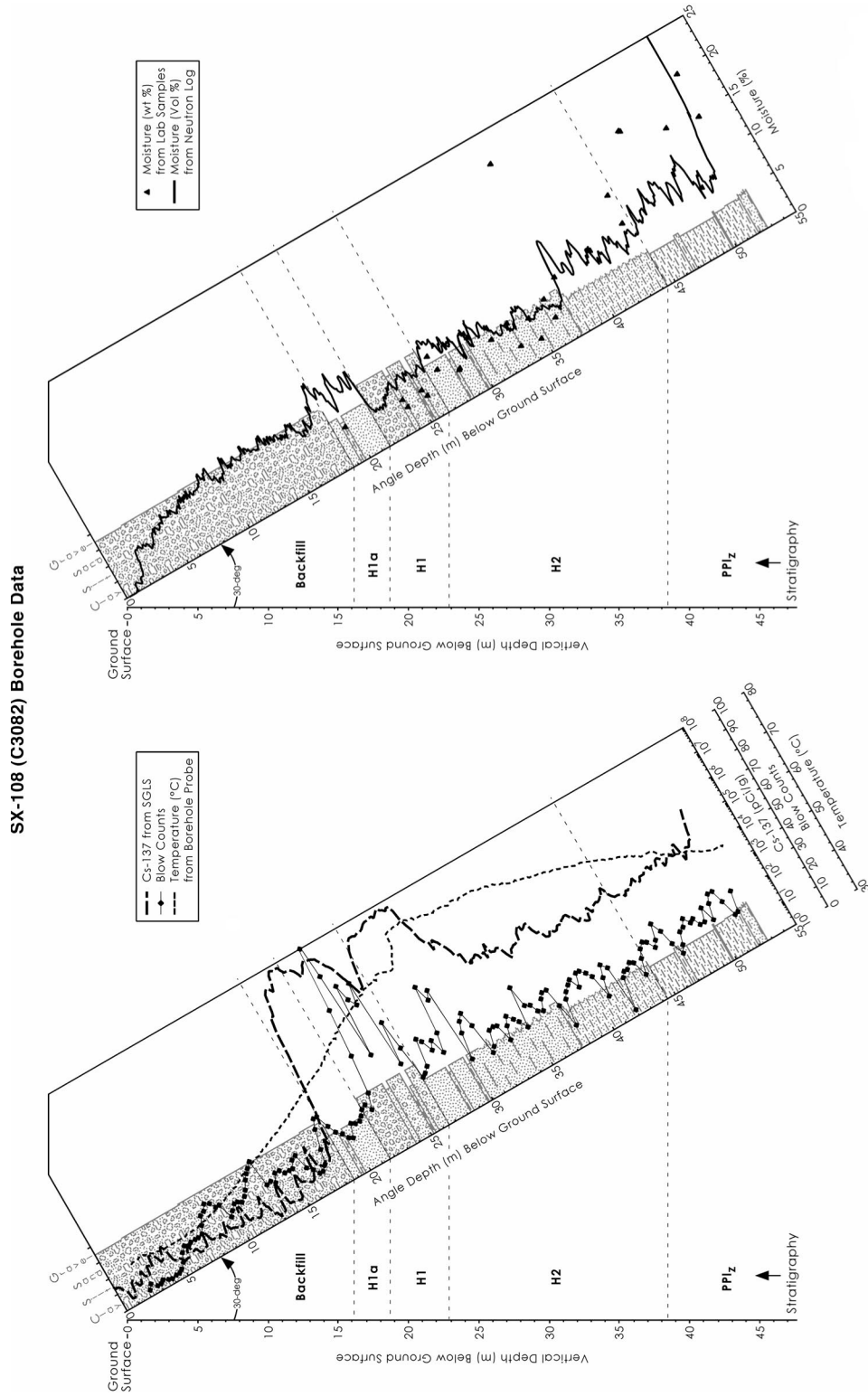
FIG. 1. Field results from the SX-108 core, including stratigraphy, counts of 137 Cs from down-hole spectral gamma logging, in situ temperature, and moisture content from down-hole neutron logging and laboratory measurements. High counts of 137 Cs were observed immediately after samples were passed through the backfill surrounding the tank (see Fig. 2). Blow counts refers to the number of hammer strikes required to advance the borehole a given distance by cable tool drilling. SGLS, spectral gamma logging system. (Reprinted from reference 46 with permission of the publisher.)
