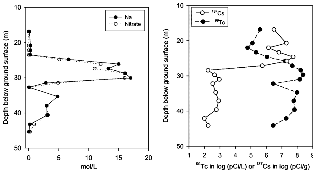
FIG. 2. Porewater concentrations of Na, NO 3 , and 99 Tc [Tc(VII)O 4 - ] in the borehole samples determined by water extraction (46) and laboratory water content measurements. Also shown for reference is the sorbed concentration of 137 Cs determined by high-resolution gamma energy analysis. (Reprinted from reference 46 with permission of the publisher.)
