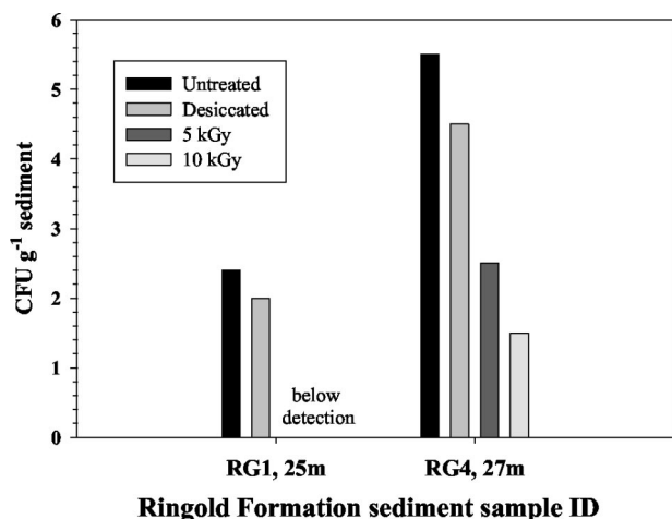
FIG. 3. Influence of acute doses of ionizing radiation ( ^{60}\text{Co} ) on populations of viable aerobic heterotrophic bacteria in uncontaminated Hanford vadose zone sediments as determined by dilution plate counts on PTYG agar medium.
