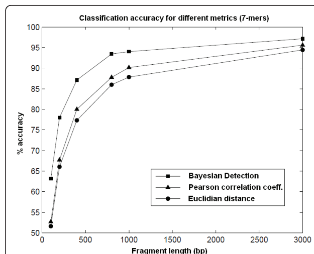
Figure 2 Classification accuracy for different distance metrics. The accuracy performance of different distance/similarity metrics for 28 taxa with varying fragment lengths is shown. The frequencies of 7-mers were used. Using the metric defined by Sandberg et al. appears to be more accurate for all fragment lengths than employing Euclidean distance and Pearson correlation coefficients.
