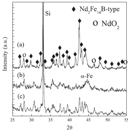
Figure 1. XRD patterns for (a) a Ti-buffered NdDyFeCoNbB + 40 wt%Fe single layer with a thickness of 640 nm on the Si substrate annealed at 600°C for 5 min; (b) a Ti(20 nm)/[NdDyFeCoNbB(16 nm) Fe(7.5 nm)] × 10/Ti(20 nm)/(Si substrate) multilayer annealed at 600°C for 20 min; (c) a Ti(10 nm)/[NdDyFeCoNbB(16 nm) Fe(1.5 nm)] × 20/Ti(10 nm)/(Si substrate) multilayer annealed at 550°C for 30 min.
