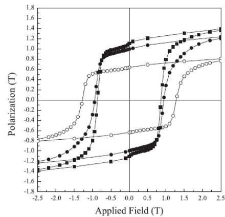
Figure 5. Room temperature hysteresis loops of a Ti(10 nm)/[NdDyFeCoNbB (16 nm)Fe(1.5 nm)] \times 20/Ti(10 nm)/(Si substrate) multilayer annealed at (■) 550°C and (●) 575°C for 30 min and a Ti(10 nm)/[NdDyFeCoNbB(320 nm)/Ti(10 nm)]/(Si substrate) layer annealed at (○) 550°C for 30 min.
