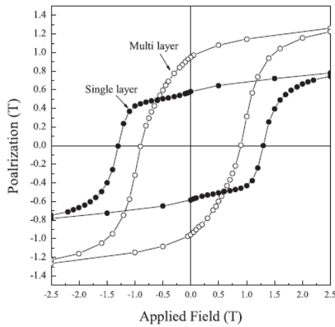
Figure 3. Room temperature hysteresis loops of a Ti(20 nm)/[NdDyFeCoNbB(16 nm) Fe(7.5 nm)] \times 10/Ti(20 nm)/(Si substrate) multilayer and a Ti(20 nm)/[NdDyFeCoNbB (160 nm)/Ti(20 nm)]/(Si substrate) annealed at 600°C for 20 min.
