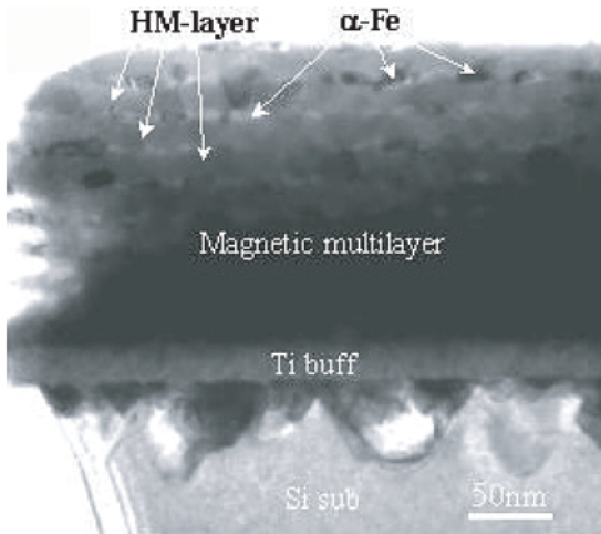
Figure 4. TEM bright-field image of the Ti(20 nm)/[NdDyFeCoNbB (16 nm)Fe(7.5 nm)] \times 10/Ti(20 nm)/(Si substrate) multilayer thin film annealed at 600°C for 20 min.
