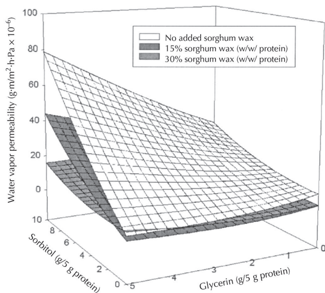
Figure 1. Response surface for the effects of sorbitol and glycerin concentrations on the water vapor permeability of sorghum wax-soy protein isolate composite films.
