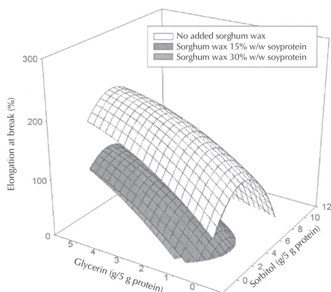
Figure 2. Response surface for the effects of sorbitol and glycerin concentrations on the elongation at break (%) of sorghum wax-soy protein isolate composite films.
