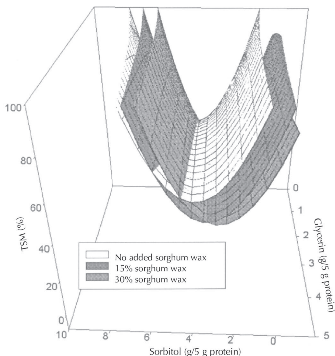
Figure 3. Response surface for the effects of sorbitol and glycerin concentrations on the total soluble matter (TSM) of sorghum wax-soy protein isolate composite films.
