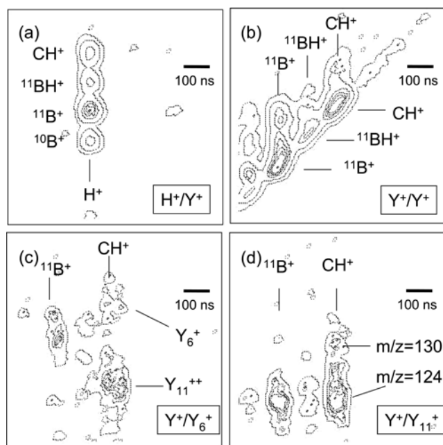
Figure 6 Detailed views represented as contour plots on sections of the photoelectron-photoion-photoion coincidence (PEPIPICO) spectrum for closo -1,2-dicarbadoecaborane (1,2- C_2B_{10}H_{12} ) recorded at 220 eV photon energy ( Y : C^+ or B^+ , X^- : 1,2- C_2B_{10}H_{12}^+ ): (a) H^+/Y^+ -regime; (b) Y^+/Y^+ -regime; (c) Y^+/Y_6^+ -regime; (d) Y^+/Y_{11}^+ -regime.
