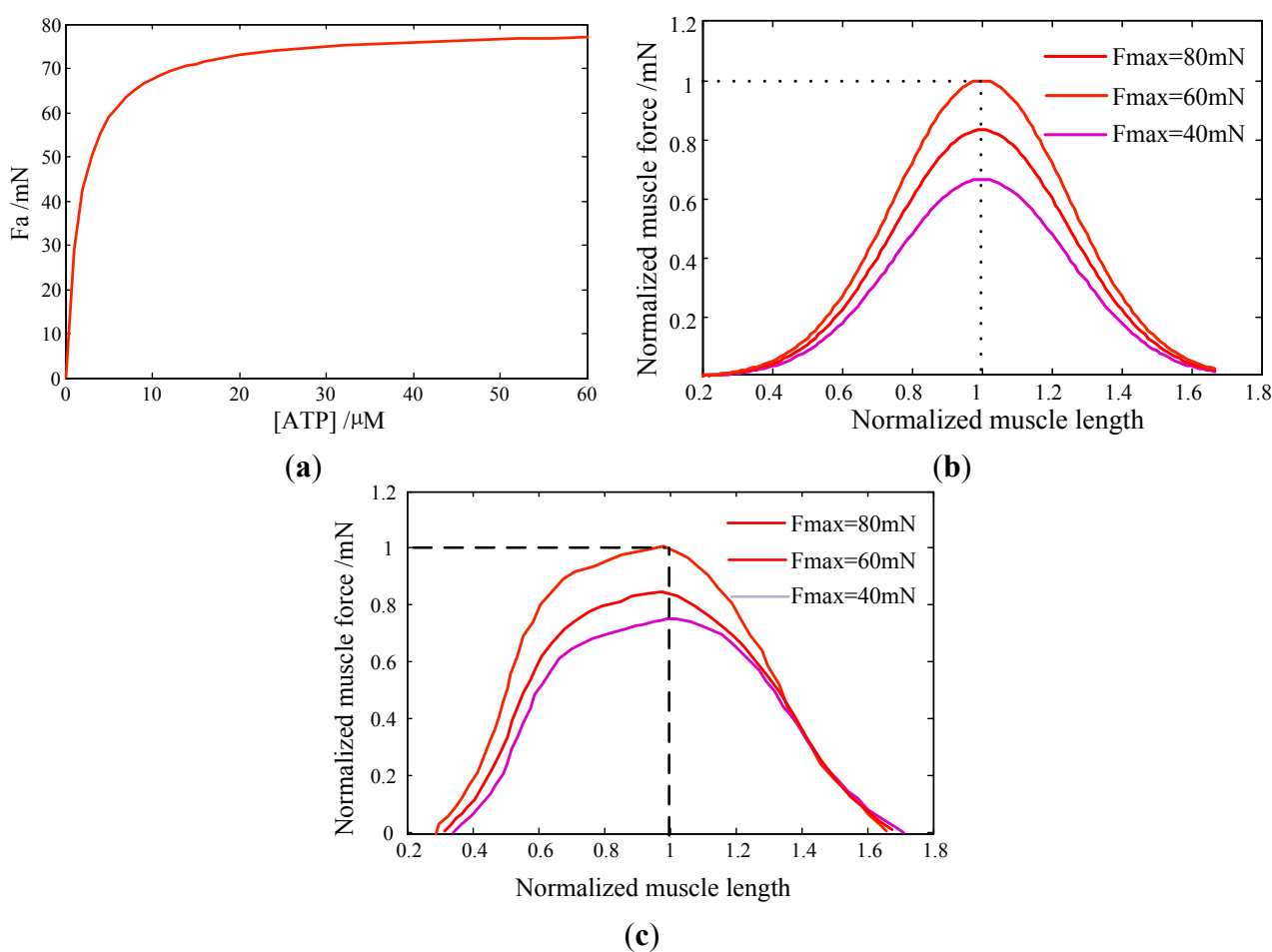
Figure 4. (a) The relationship between active contraction force and [ATP]; Active force-length curves, normalized by the maximum muscle force and optimal fiber length, respectively, calculated from either our model (b) or the Hill model (c).
