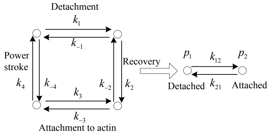
Figure 2. The simplification of working cycle of myosin motor.
