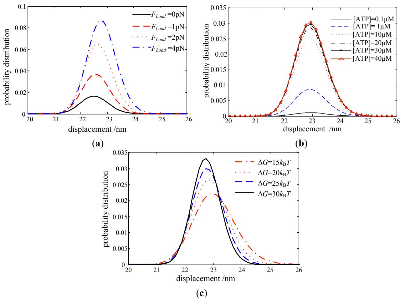
Figure 3. Probability density distribution of the molecular motor in relation to (a) various loads with [ATP] = 30 micromolar; (b) ATP concentration with load F_{Load} = 6 pN; and (c) potential profiles with F_{Load} = 6 pN.
