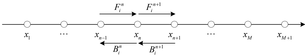
Figure 1. The spatial discretization and jump rates between two sites.
