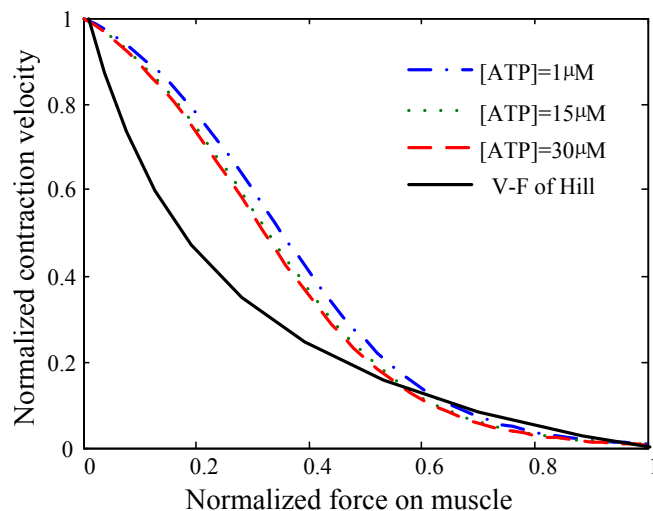
Figure 5. The normalized V-F curves.
